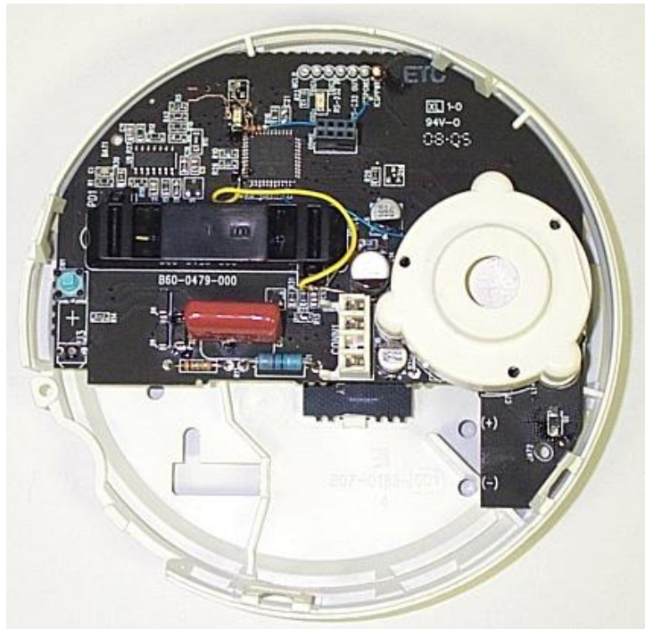
RF PCB removed
