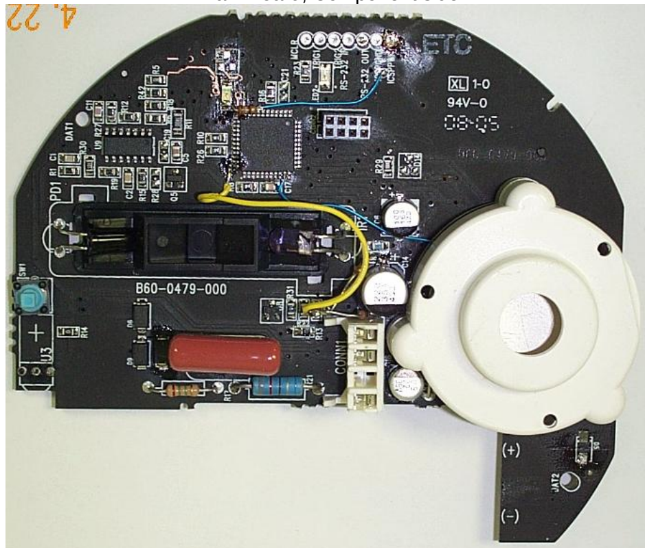
Main Board; Component side
