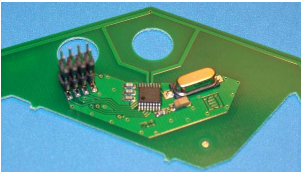
RF PCB Bottom
