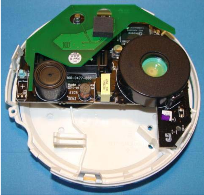
EUT With cover off
