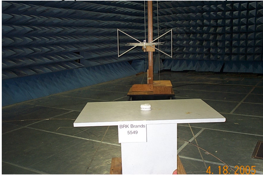
Photographs of Radiated Emissions Test Setup
