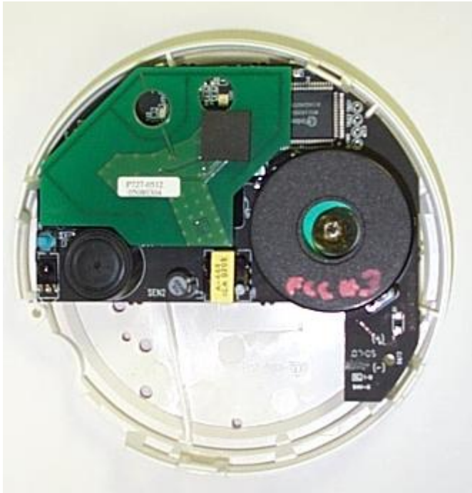
Bottom Cover
