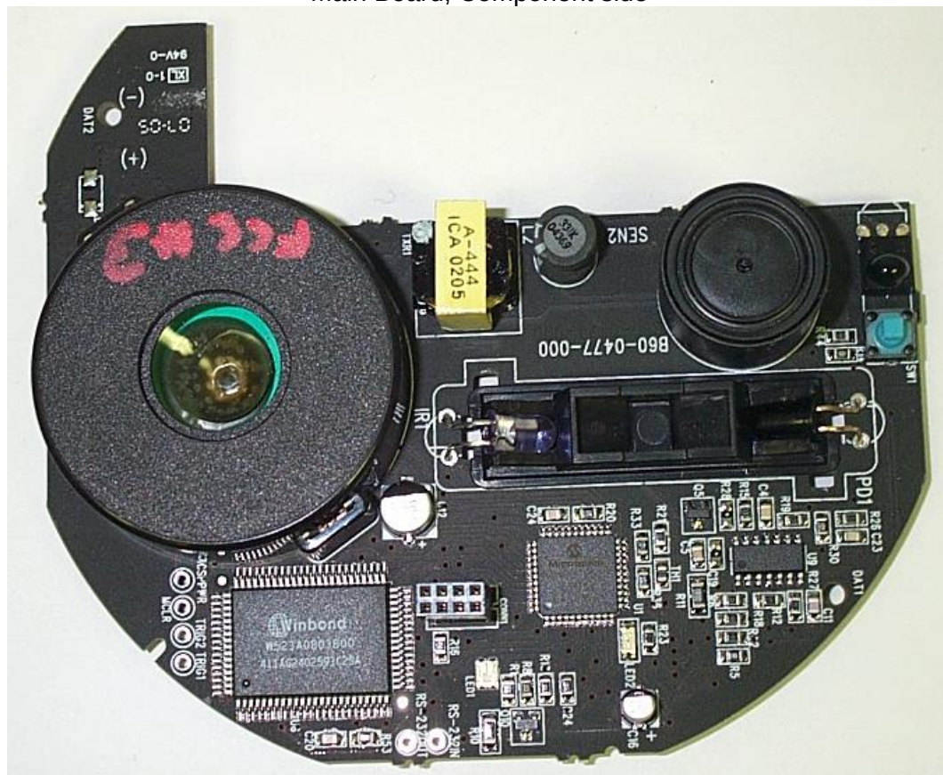
Main Board; Component side
