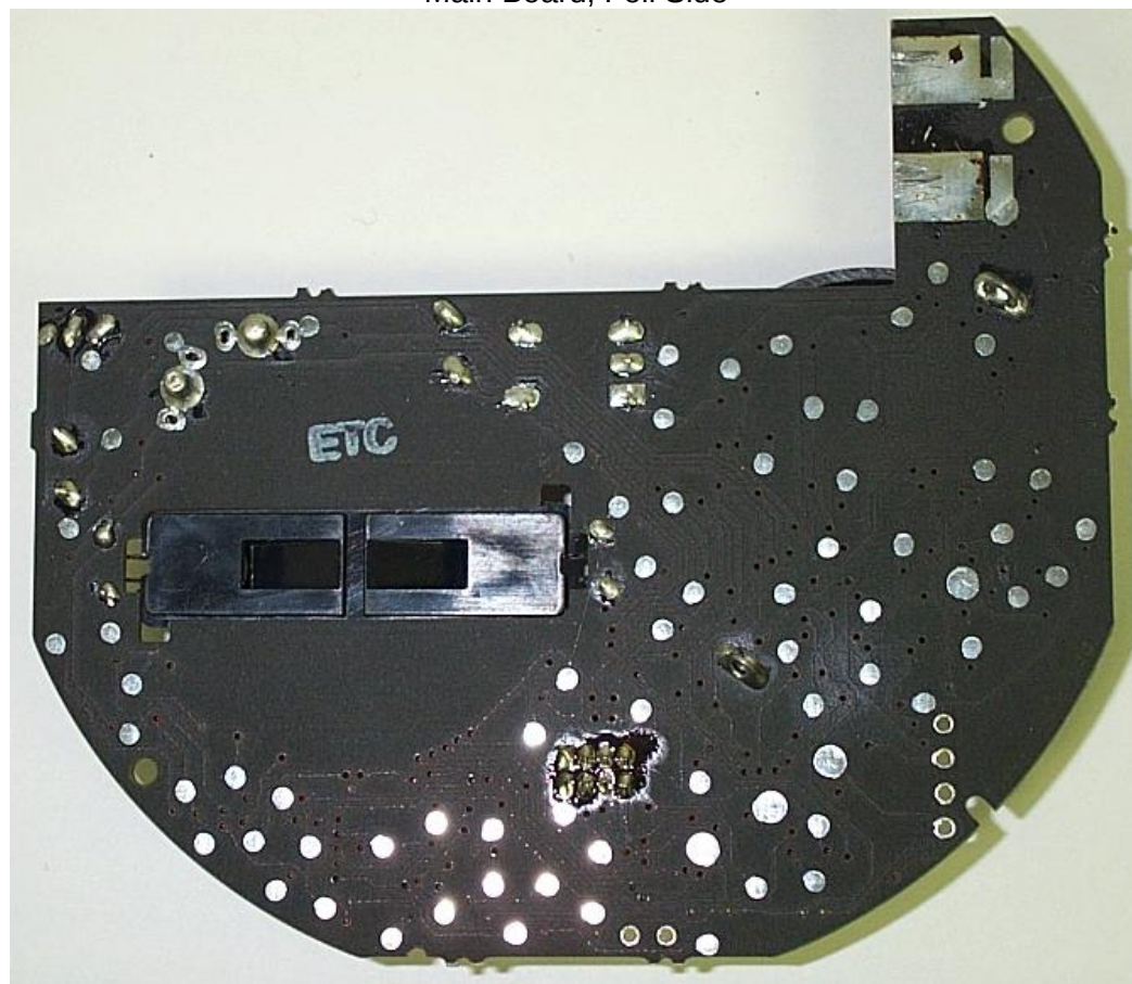
Main Board; Foil Side
