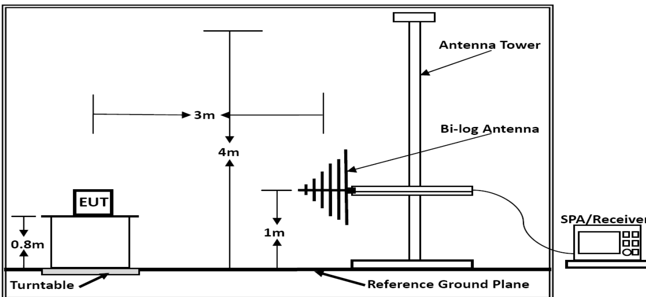
Below 1GHz
