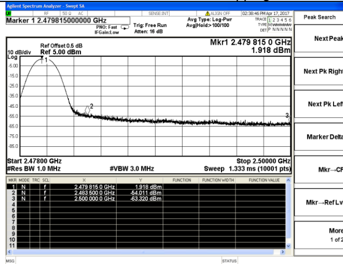
Channel 78 / 2480 MHz – Non-Hopping – Peak
