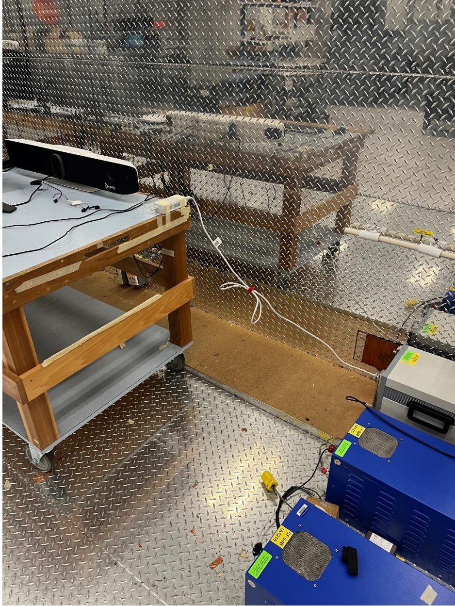
Conducted Emissions Close Up on LISN
