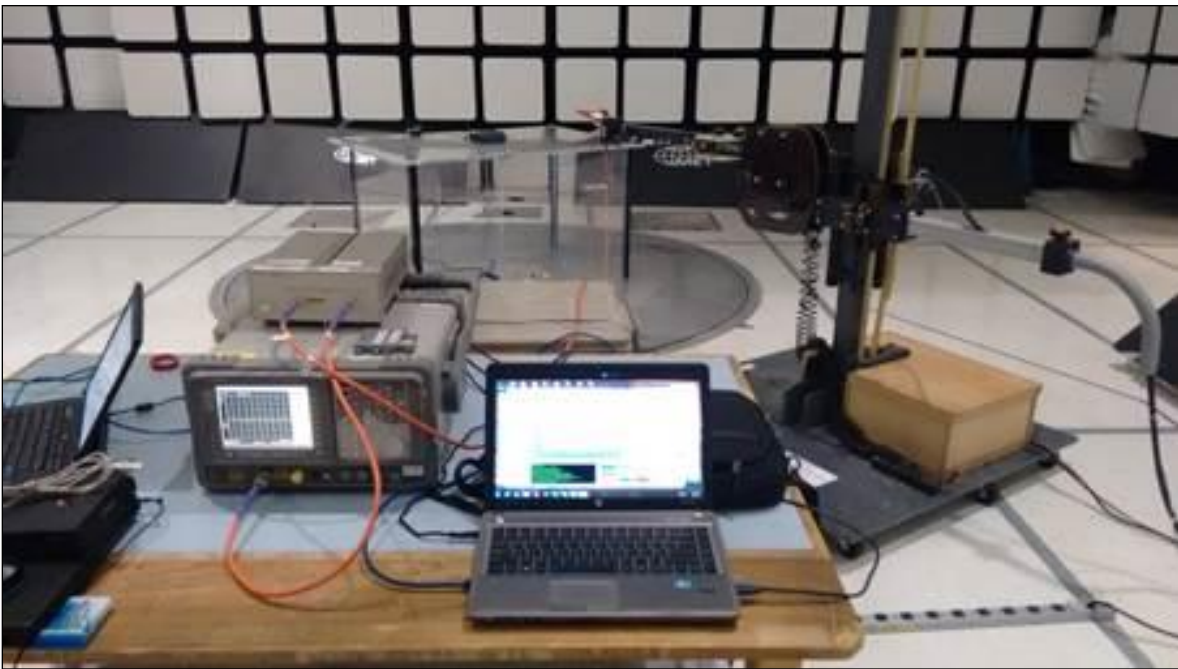
Photograph 2. Radiated Spurious Emissions, Above 1 GHz, Test Setup
