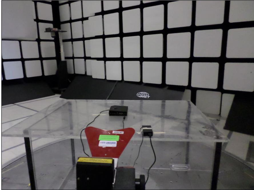
Photograph 3. Radiated Emissions, Above 1 GHz, Test Setup
