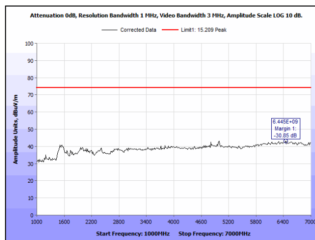
Plot 6. Radiated Spurious Emissions, Low Channel, BLE, 1 GHz – 7 GHz, Peak
