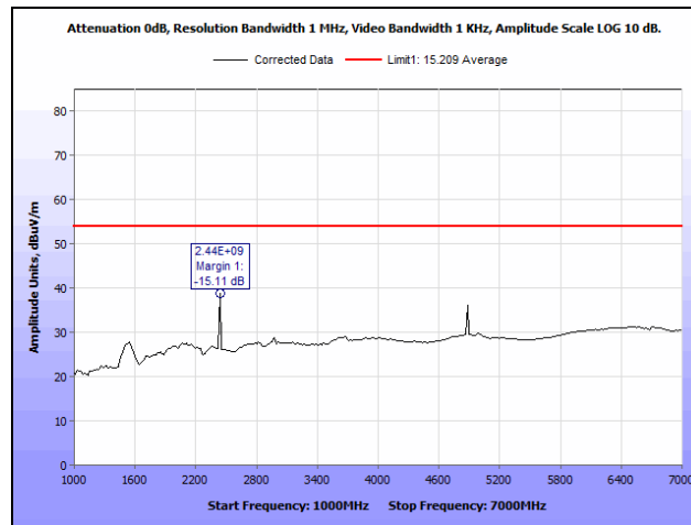
Plot 10. Radiated Spurious Emissions, Mid Channel, BLE, 1 GHz – 7 GHz, Average
