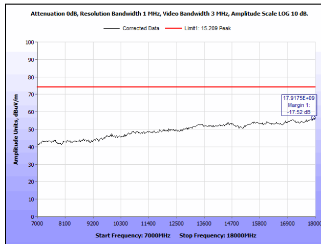
Plot 8. Radiated Spurious Emissions, Low Channel, BLE, 7 GHz – 18 GHz, Peak
