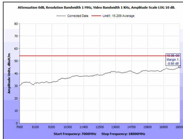
Plot 7. Radiated Spurious Emissions, Low Channel, BLE, 7 GHz – 18 GHz, Average
