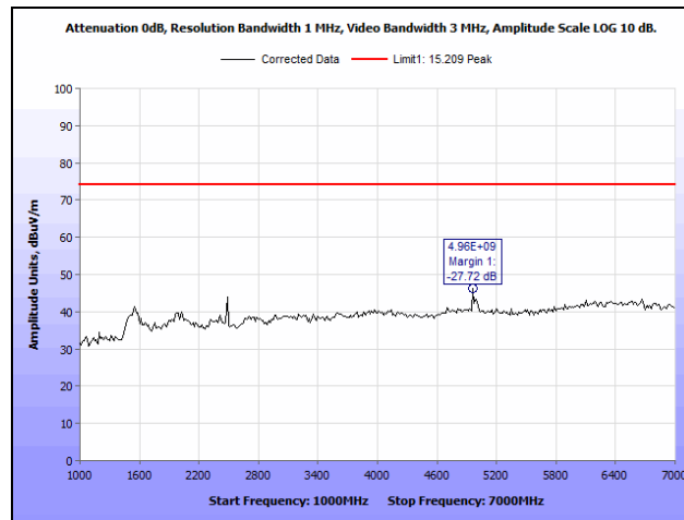
Plot 16. Radiated Spurious Emissions, High Channel, BLE, 1 GHz – 7 GHz, Peak
