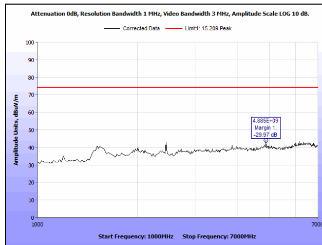
Plot 11. Radiated Spurious Emissions, Mid Channel, BLE, 1 GHz – 7 GHz, Peak
