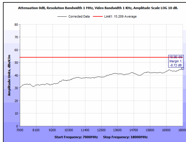
Plot 17. Radiated Spurious Emissions, High Channel, BLE, 7 GHz – 18 GHz, Average
