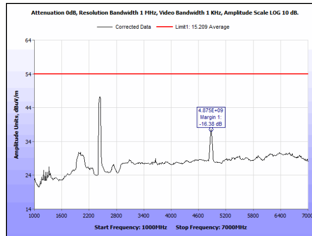
Plot 76. Radiated Spurious Emissions, Mid Channel, 802.11n 40 MHz, Both Chains, 1 GHz – 7 GHz, Average
