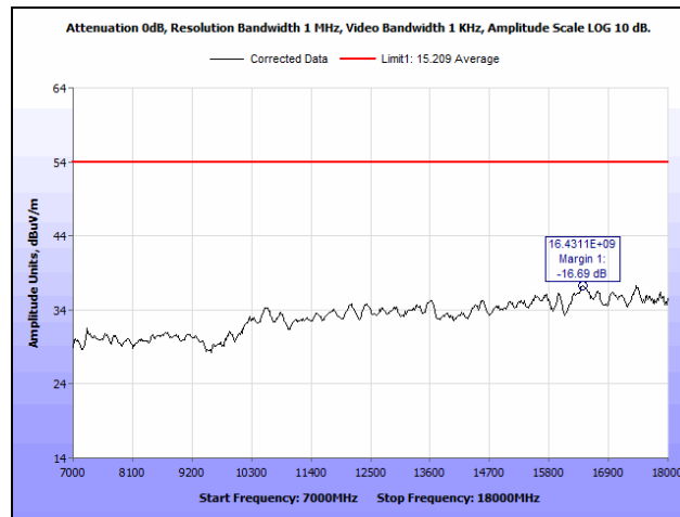
Plot 73. Radiated Spurious Emissions, Low Channel, 802.11n 40 MHz, Both Chains, 7 GHz – 18 GHz, Average
