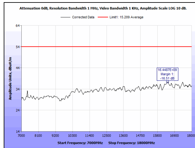
Plot 53. Radiated Spurious Emissions, High Channel, 802.11g 20 MHz, Both Chains, 7 GHz – 18 GHz, Average
