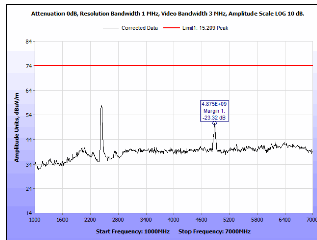
Plot 77. Radiated Spurious Emissions, Mid Channel, 802.11n 40 MHz, Both Chains, 1 GHz – 7 GHz, Peak
