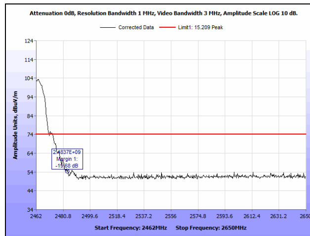
Plot 88. Radiated Restricted Band Edge, High Channel, 802.11b 20 MHz, Both Chains, Peak
