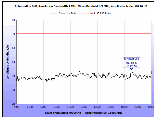
Plot 34. Radiated Spurious Emissions, Mid Channel, 802.11b 20 MHz, Both Chains, 7 GHz – 18 GHz, Peak
