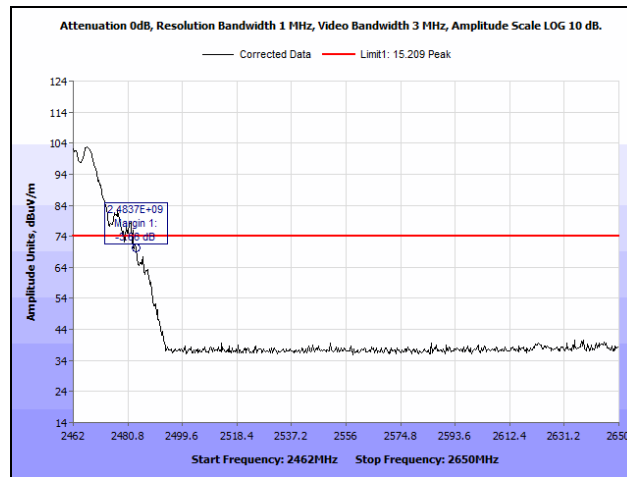
Plot 92. Radiated Restricted Band Edge, High Channel, 802.11g 20 MHz, Both Chains, Peak
