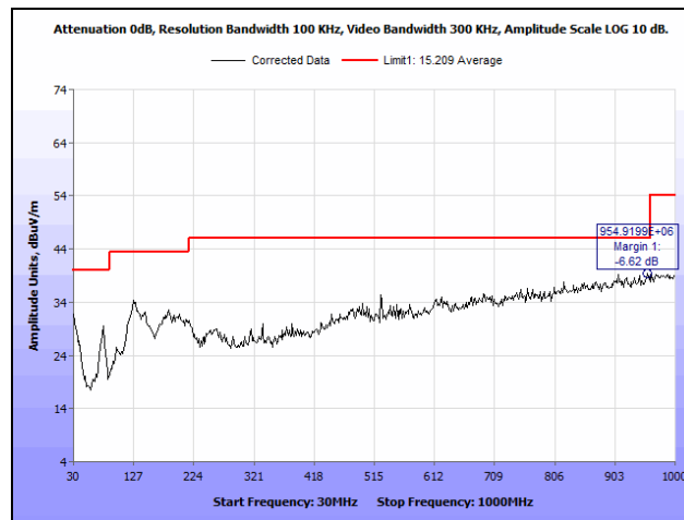
Plot 65. Radiated Spurious Emissions, High Channel, 802.11n 20 MHz, Both Chains, 30 MHz – 1 GHz
