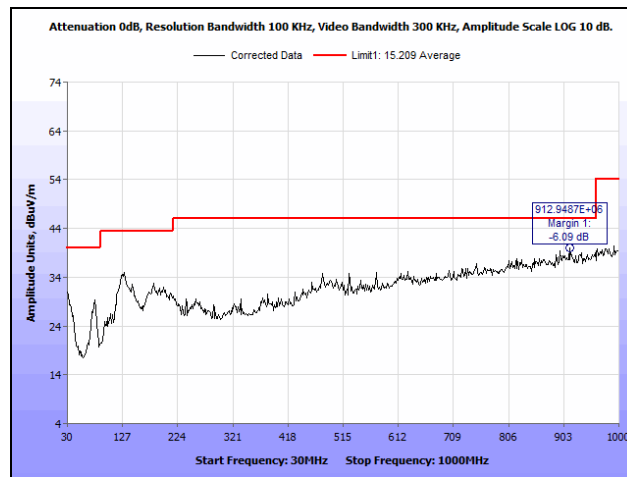
Plot 50. Radiated Spurious Emissions, High Channel, 802.11g 20 MHz, Both Chains, 30 MHz – 1 GHz
