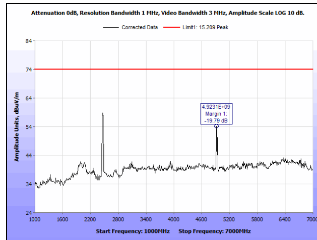
Plot 52. Radiated Spurious Emissions, High Channel, 802.11g 20 MHz, Both Chains, 1 GHz – 7 GHz, Peak
