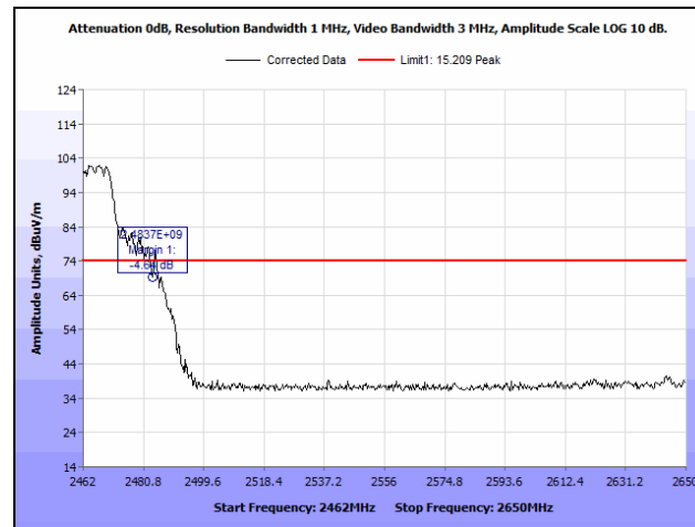
Plot 96. Radiated Restricted Band Edge, High Channel, 802.11n 20 MHz, Both Chains, Peak
