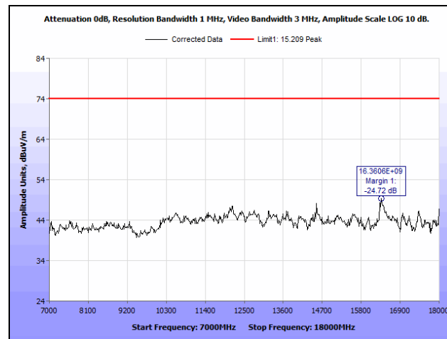
Plot 59. Radiated Spurious Emissions, Low Channel, 802.11n 20 MHz, Both Chains, 7 GHz – 18 GHz, Peak
