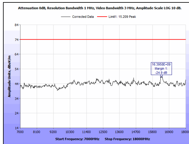
Plot 74. Radiated Spurious Emissions, Low Channel, 802.11n 40 MHz, Both Chains, 7 GHz – 18 GHz, Peak
