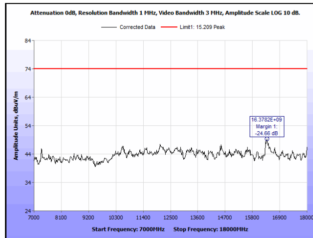
Plot 49. Radiated Spurious Emissions, Mid Channel, 802.11g 20 MHz, Both Chains, 7 GHz – 18 GHz, Peak
