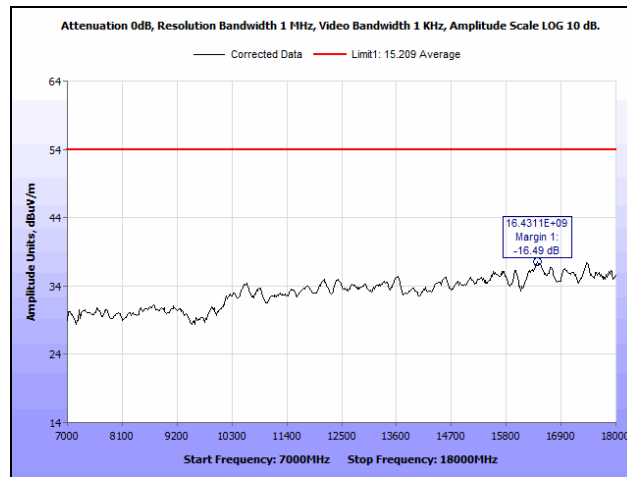
Plot 43. Radiated Spurious Emissions, Low Channel, 802.11g 20 MHz, Both Chains, 7 GHz – 18 GHz, Average
