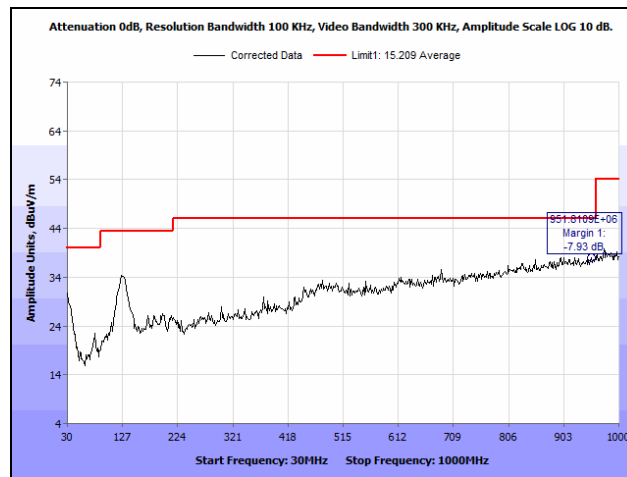
Plot 35. Radiated Spurious Emissions, High Channel, 802.11b 20 MHz, Both Chains, 30 MHz – 1 GHz
