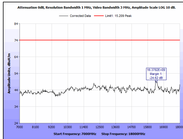
Plot 64. Radiated Spurious Emissions, Mid Channel, 802.11n 20 MHz, Both Chains, 7 GHz – 18 GHz, Peak
