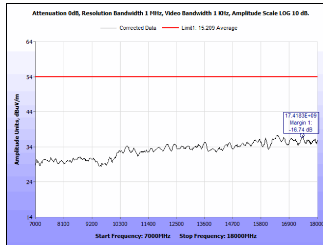
Plot 58. Radiated Spurious Emissions, Low Channel, 802.11n 20 MHz, Both Chains, 7 GHz – 18 GHz, Average
