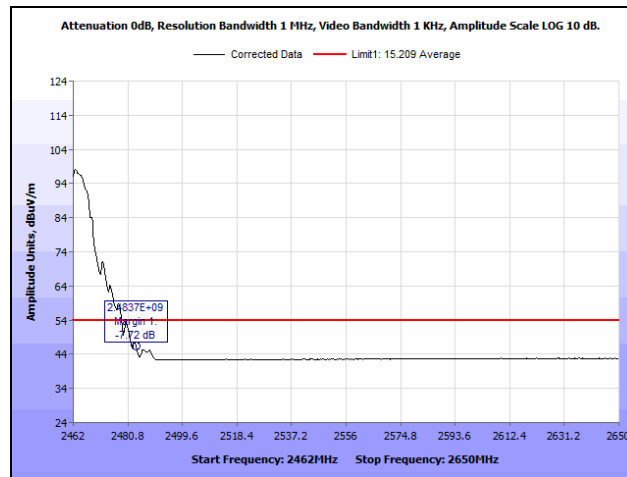
Plot 87. Radiated Restricted Band Edge, High Channel, 802.11b 20 MHz, Both Chains, Average
