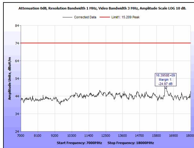
Plot 44. Radiated Spurious Emissions, Low Channel, 802.11g 20 MHz, Both Chains, 7 GHz – 18 GHz, Peak
