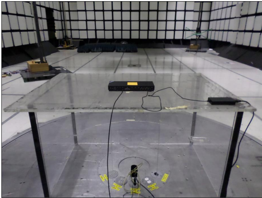
Photograph 3. Radiated Spurious Emissions, Test Setup, Below 1 GHz, Rear View
