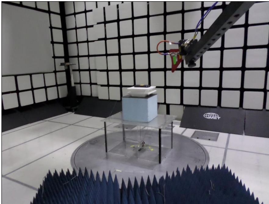
Photograph 7. Radiated Spurious Emissions, Test Setup, 1 GHz – 18 GHz, Antenna View
