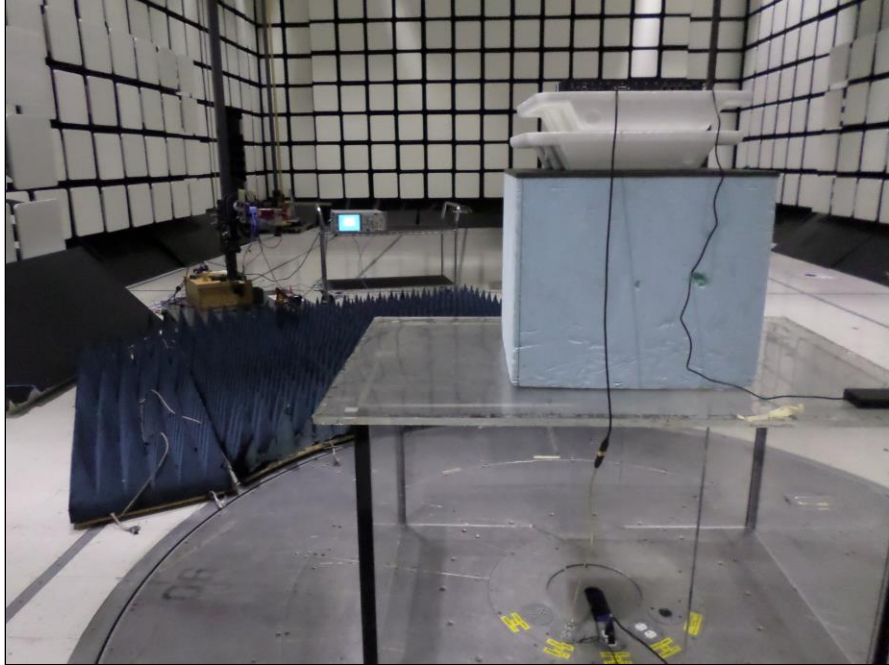
Photograph 8. Radiated Spurious Emissions, Test Setup, Above 18 GHz, Rear View
