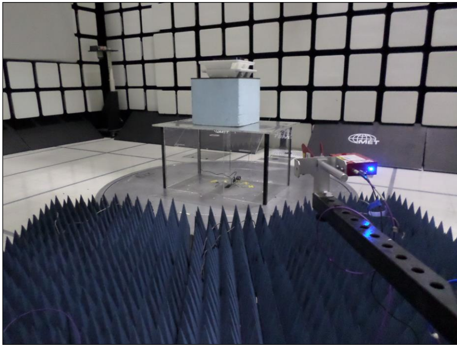
Photograph 9. Radiated Spurious Emissions, Test Setup, Above 18 GHz, Antenna View
