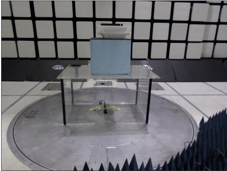
Photograph 5. Radiated Spurious Emissions, Test Setup, Above 1 GHz, Front View
