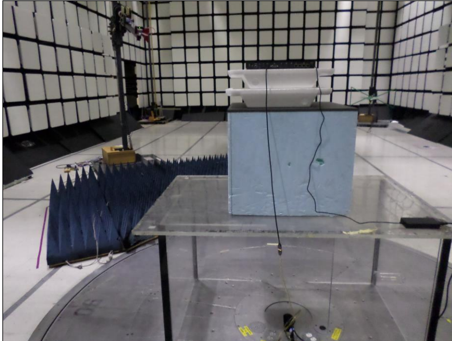
Photograph 6. Radiated Spurious Emissions, Test Setup, 1 GHz – 18 GHz, Rear View
