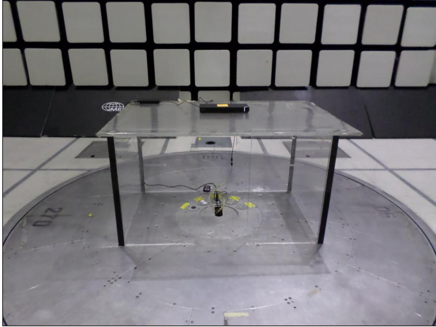
Photograph 2. Radiated Spurious Emissions, Test Setup, Below 1 GHz, Front View
