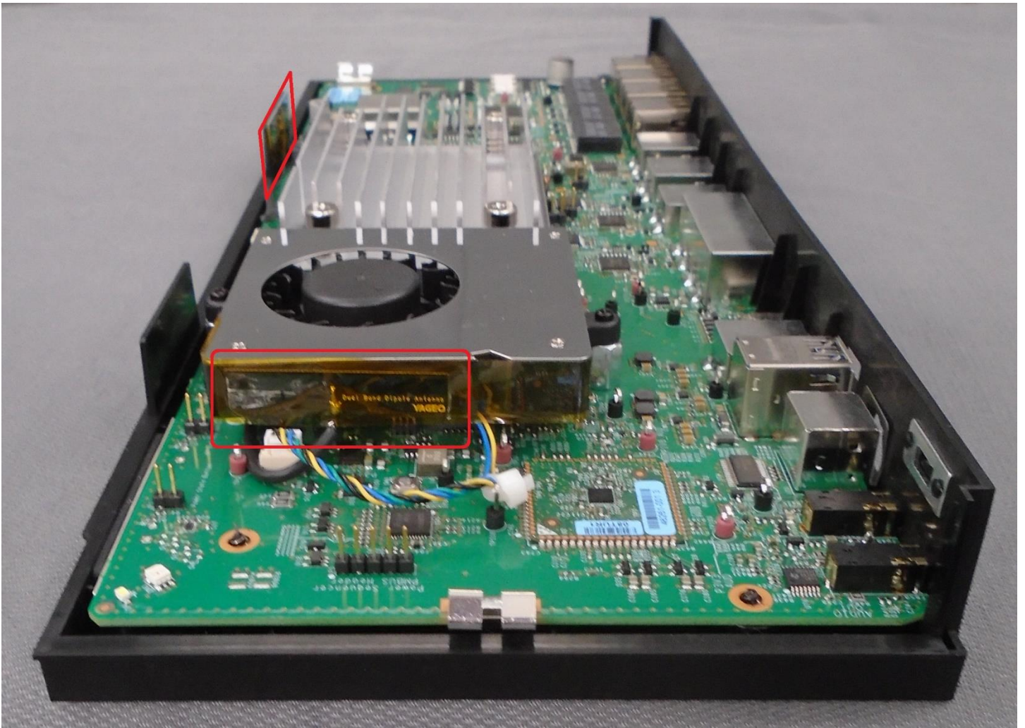
Antenna Locations
