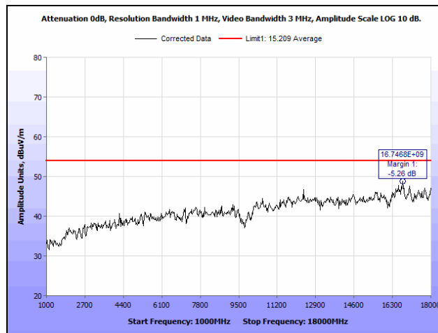
Plot 10. Radiated Spurious Emissions, Low Channel, 1 GHz – 18 GHz
