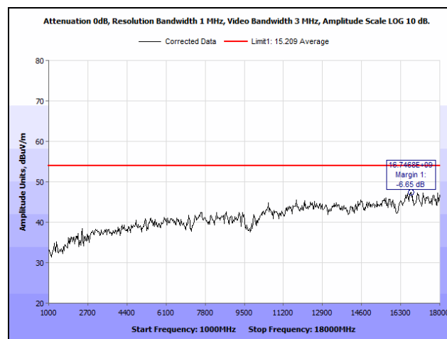
Plot 14. Radiated Spurious Emissions, High Channel, 1 GHz – 18 GHz
