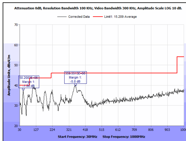
Plot 11. Radiated Spurious Emissions, Mid Channel, 30 MHz – 1 GHz
