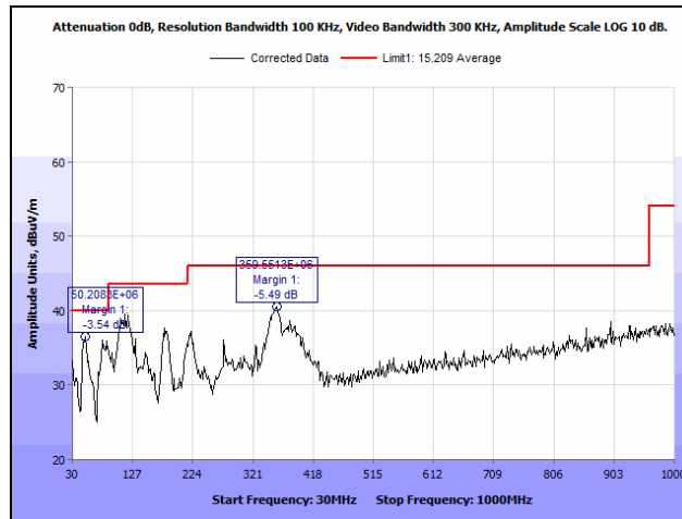
Plot 9. Radiated Spurious Emissions, Low Channel, 30 MHz – 1 GHz
