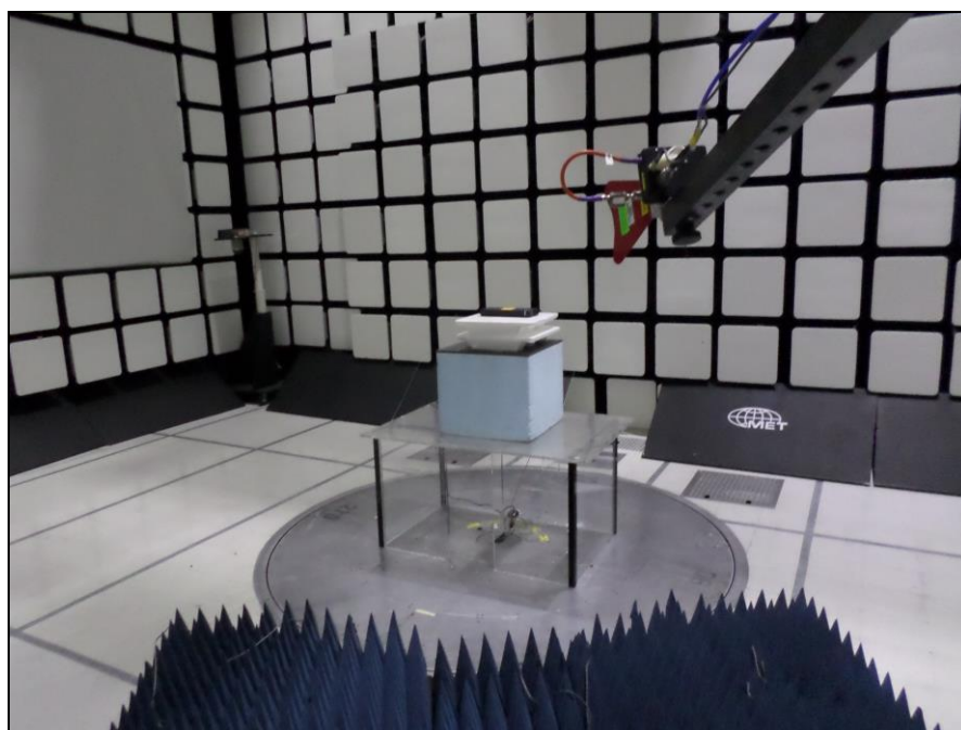
Photograph 8. Radiated Spurious Emissions, Test Setup, 1 GHz – 18 GHz, Antenna View
