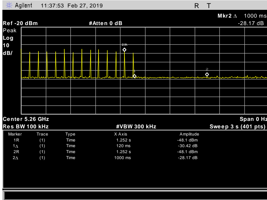
Plot 2. Channel Close Time, 5.26 GHz
