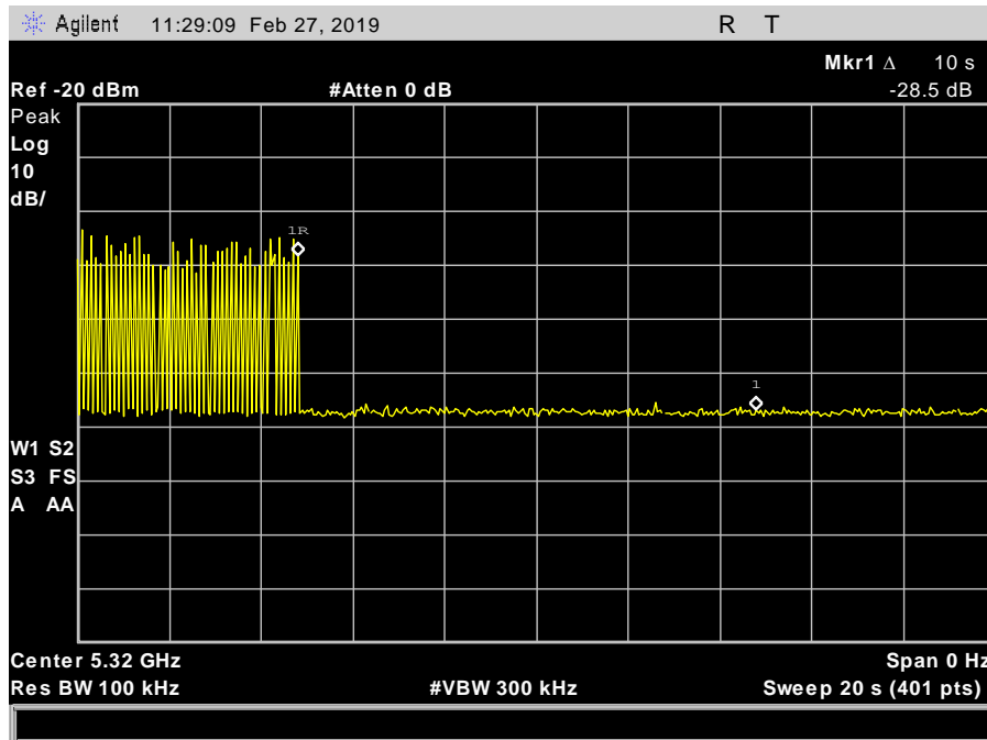
Plot 3. Channel Move Time, 5.32 GHz
