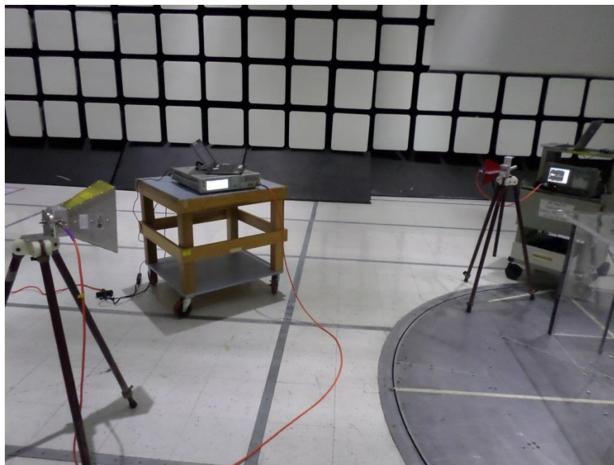
Photograph 3. DFS Calibration Setup
