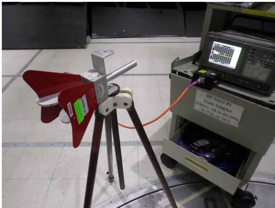
Photograph 5. DFS Receiving Antenna Setup
