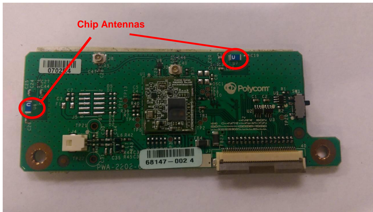
Figure 2. Chip Antenna on EUT
