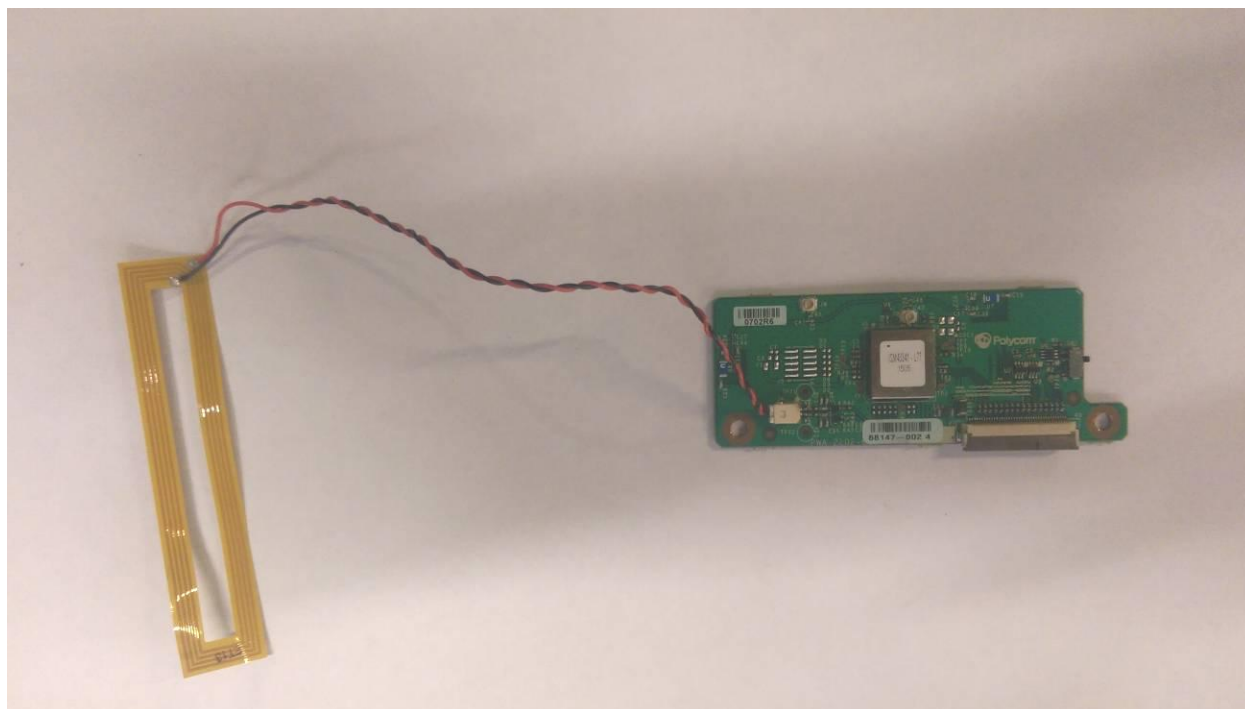
Figure 1. NFC Antenna for P008 SIP Application Module
