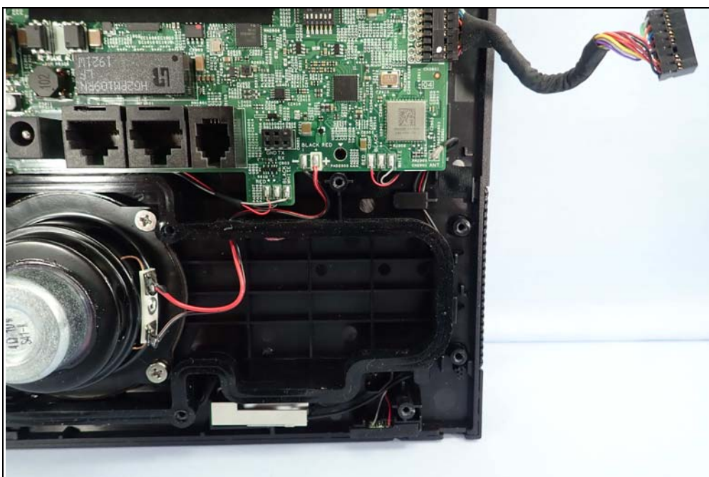
PCB antenna
