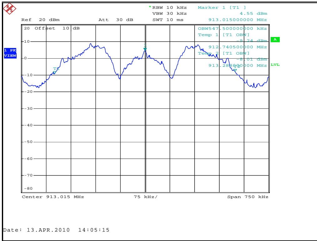
Figure 7.4.2-5: 99% Bandwidth Plot – Mid Channel
