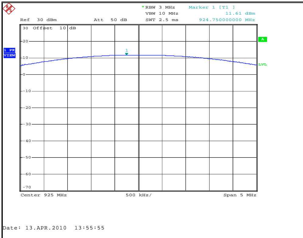
Figure 7.5.2-3: Peak Power Output – High Channel
