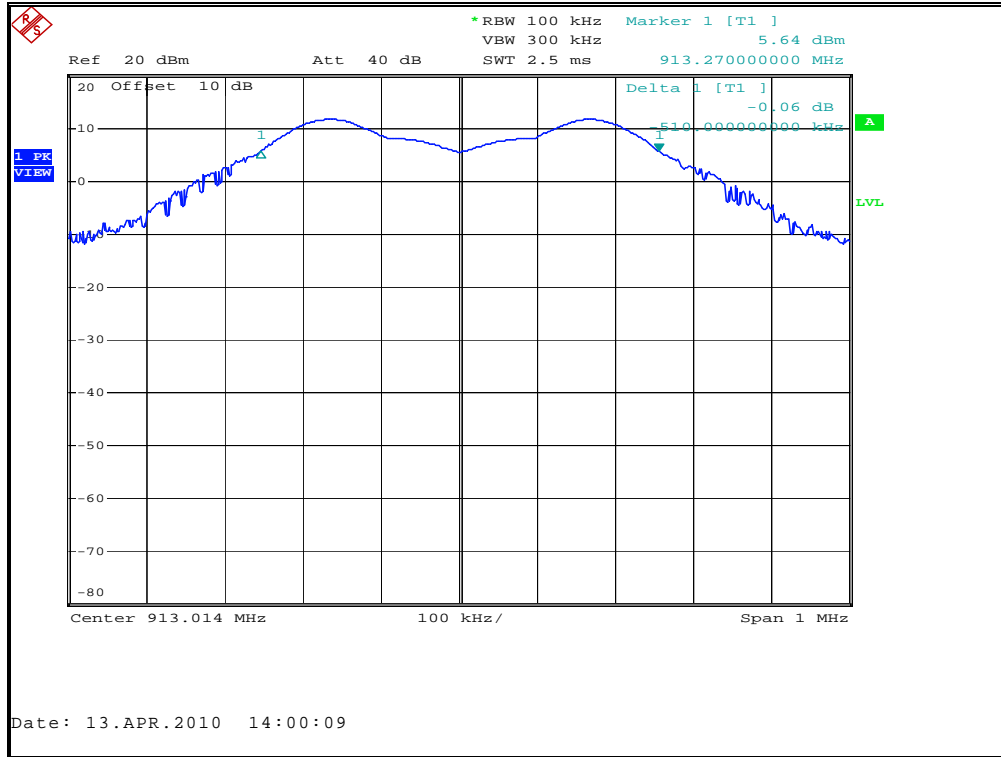
Figure 7.4.2-2: 6dB Bandwidth Plot – Mid Channel
