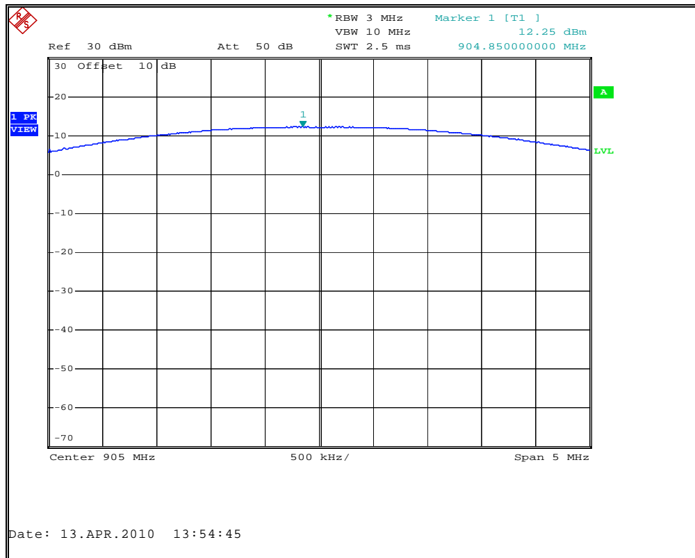
Figure 7.5.2-1: Peak Power Output – Low Channel
