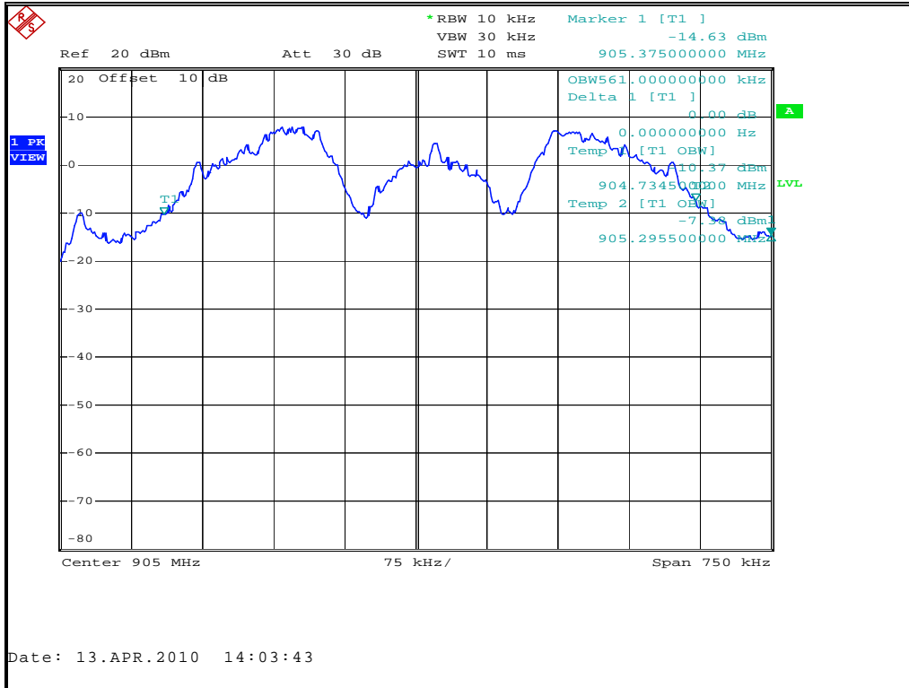
Figure 7.4.2-4: 99% Bandwidth Plot – Low Channel
