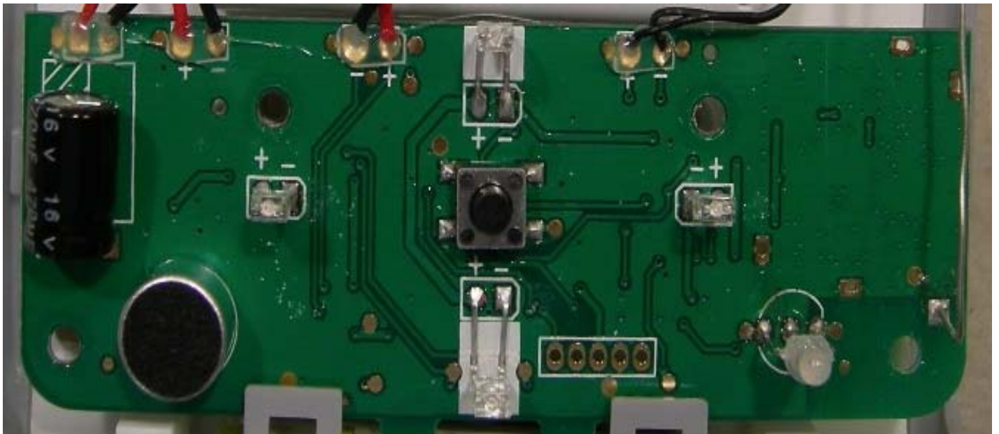
Figure 2: PCB - Back
