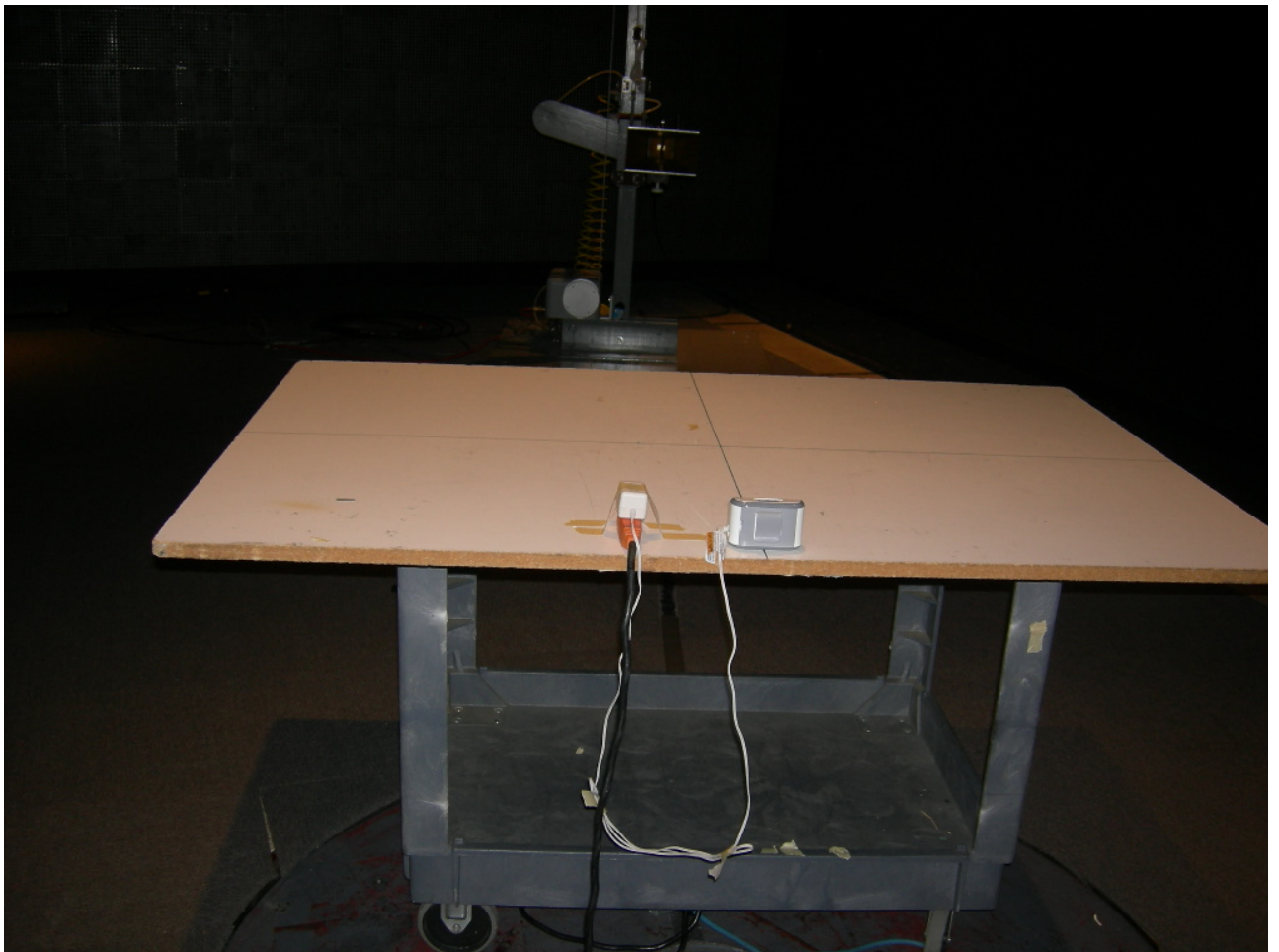
Figure 1: Radiated Emissions
