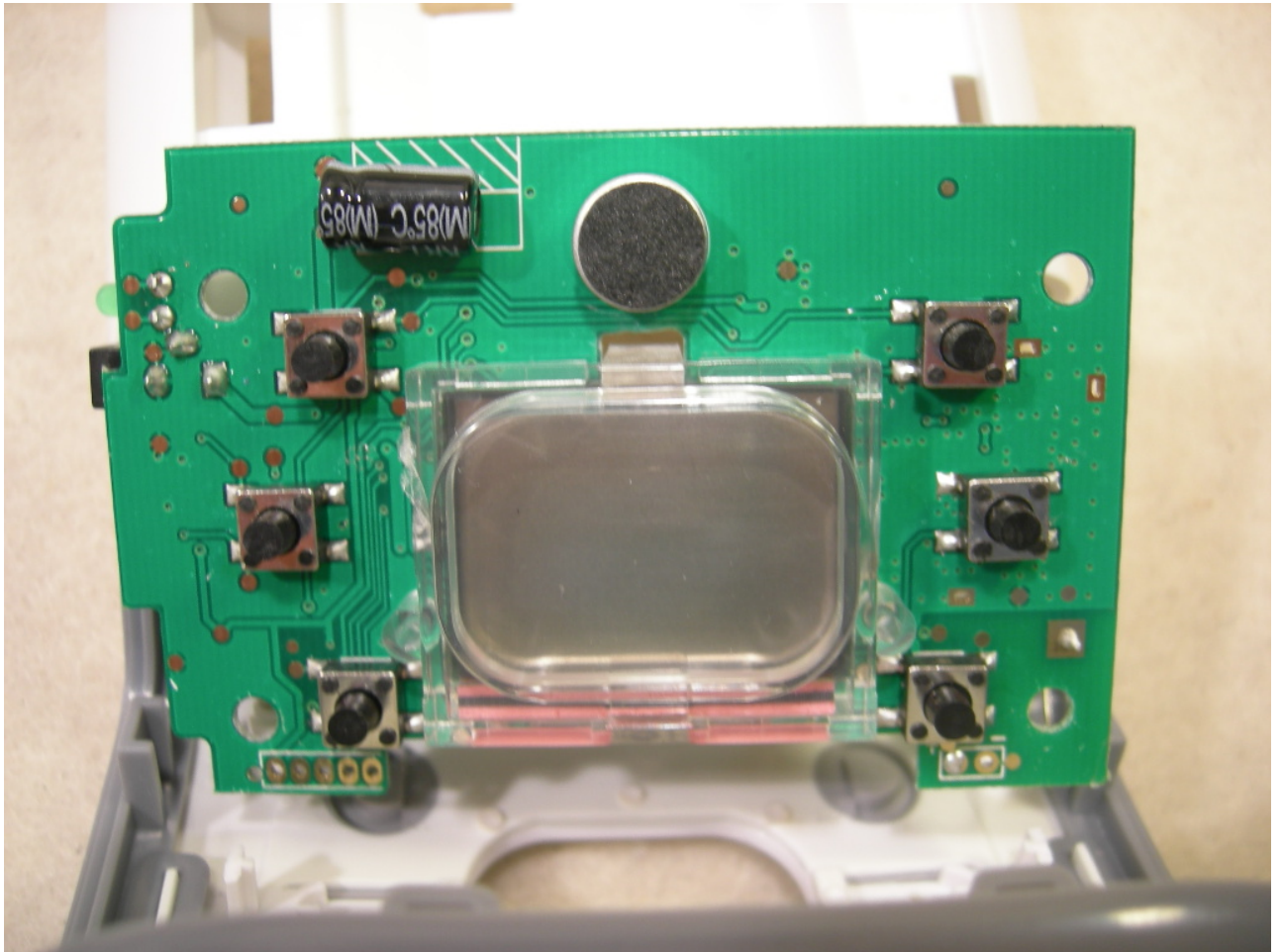
Figure 2: PCB - Back
