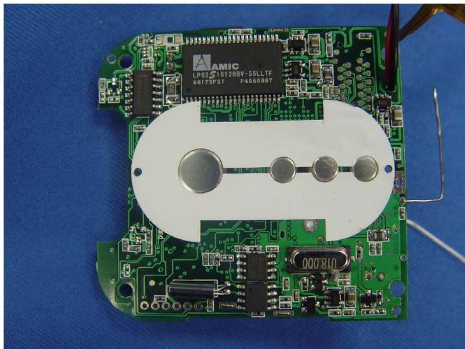
Figure 10 Inside of the EUT
