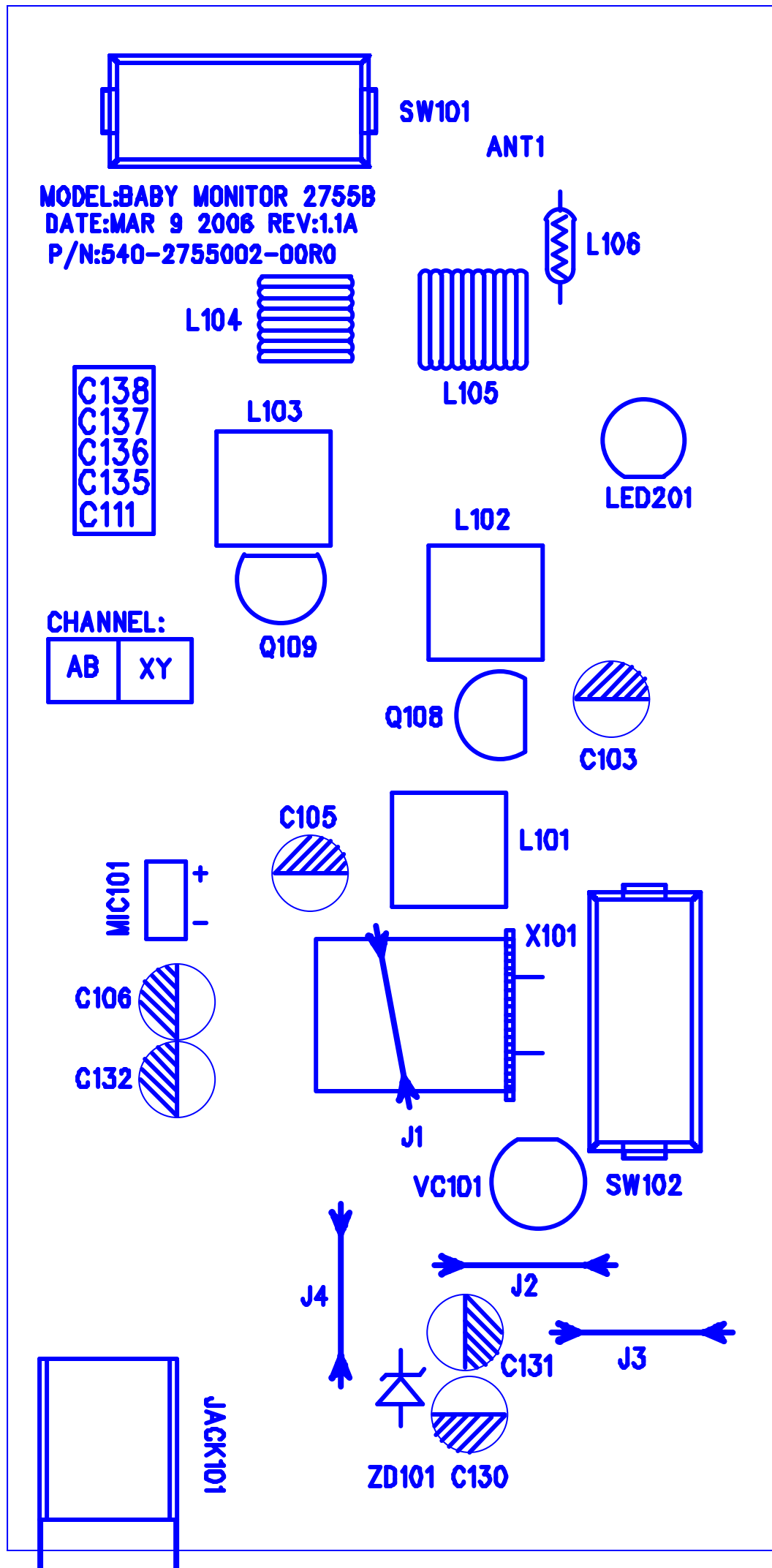
TOP SILKSCREEN SIDE
