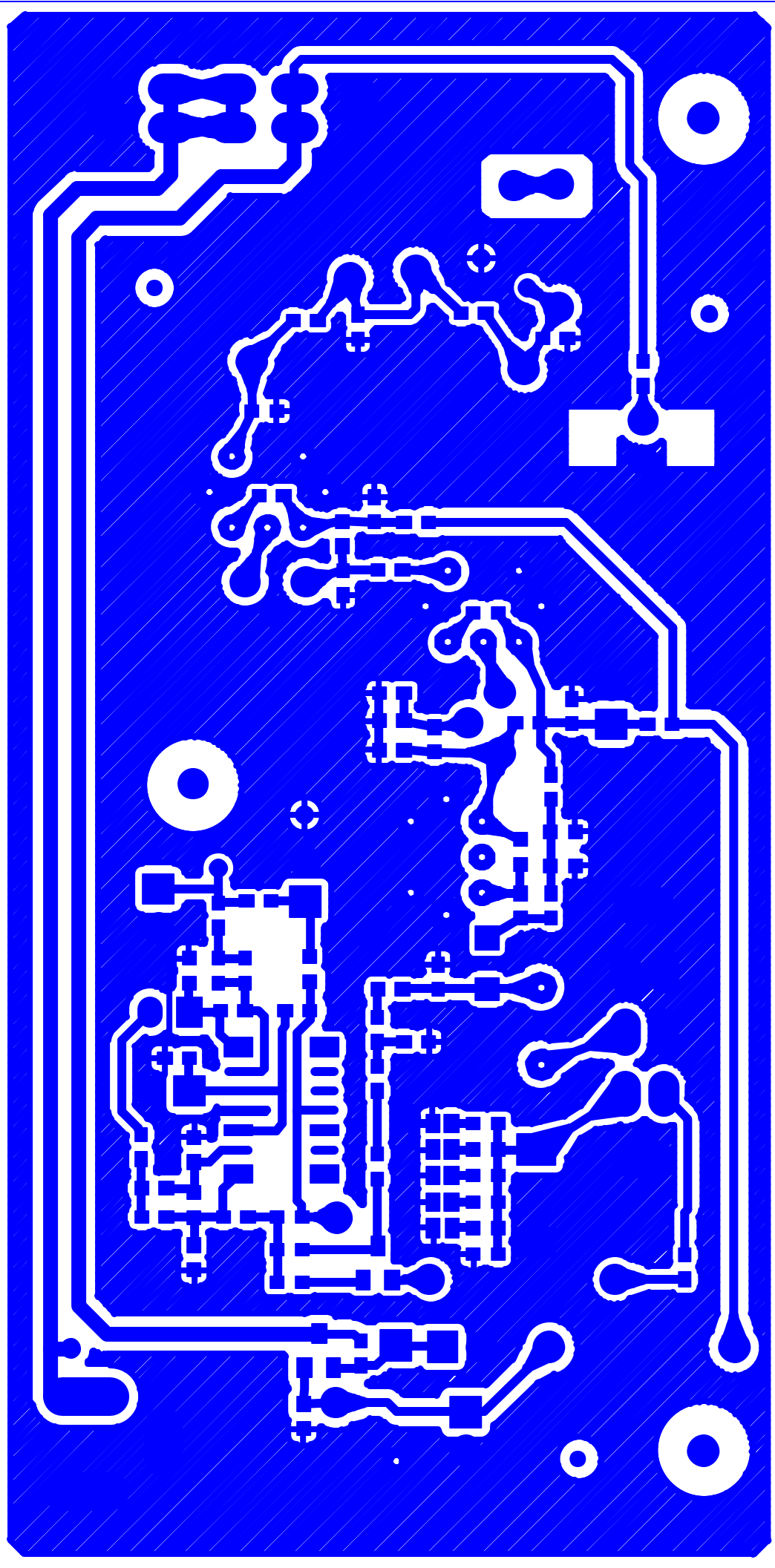
BOTTOM COPPER SIDE
