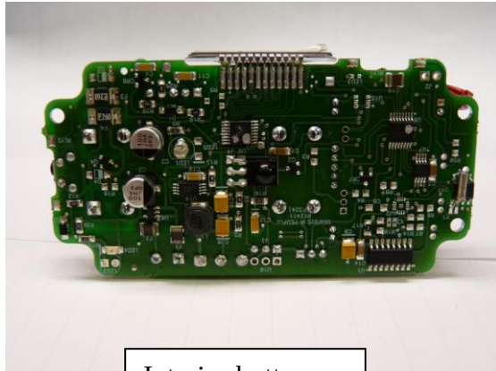
Interior bottom
