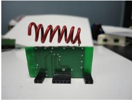
Figure 1 418MHz PCB Side
