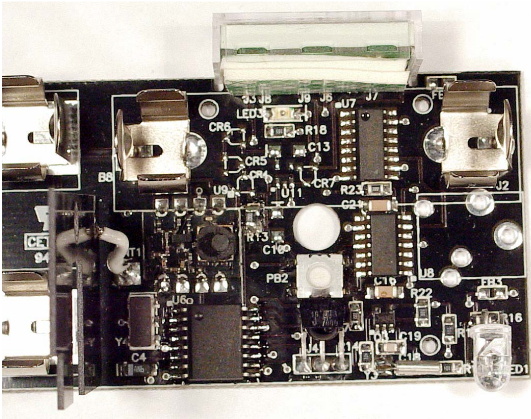
Component view of the IR Counter Transmitter, Model Point Sensor IR Counter
