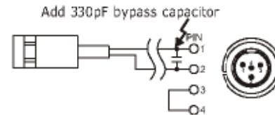
Add 330pF bypass capacitor
