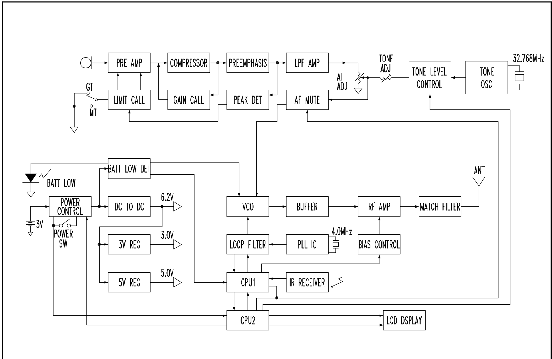
BLOCK DIAGRAM
