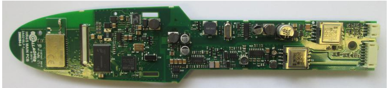
Main PCB (Top Side)
