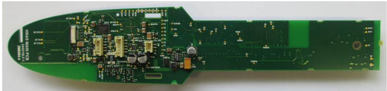
Main PCB (Bottom Side)
