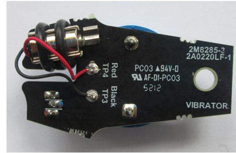
Vibrator PCB (Solder Side)
