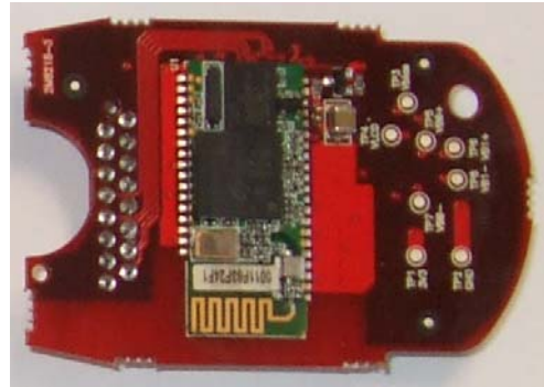
Buzzer PCB - Bottom Side
