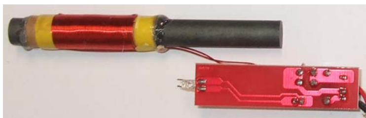
Internal Assembly
