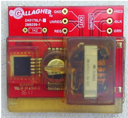
Power Line Filter PCB - Component Side
