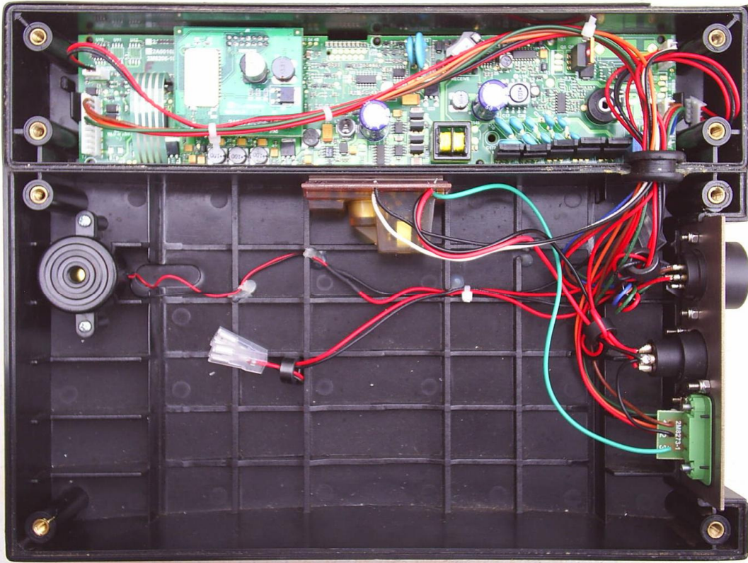
R Reader - Internal Assembly 1
