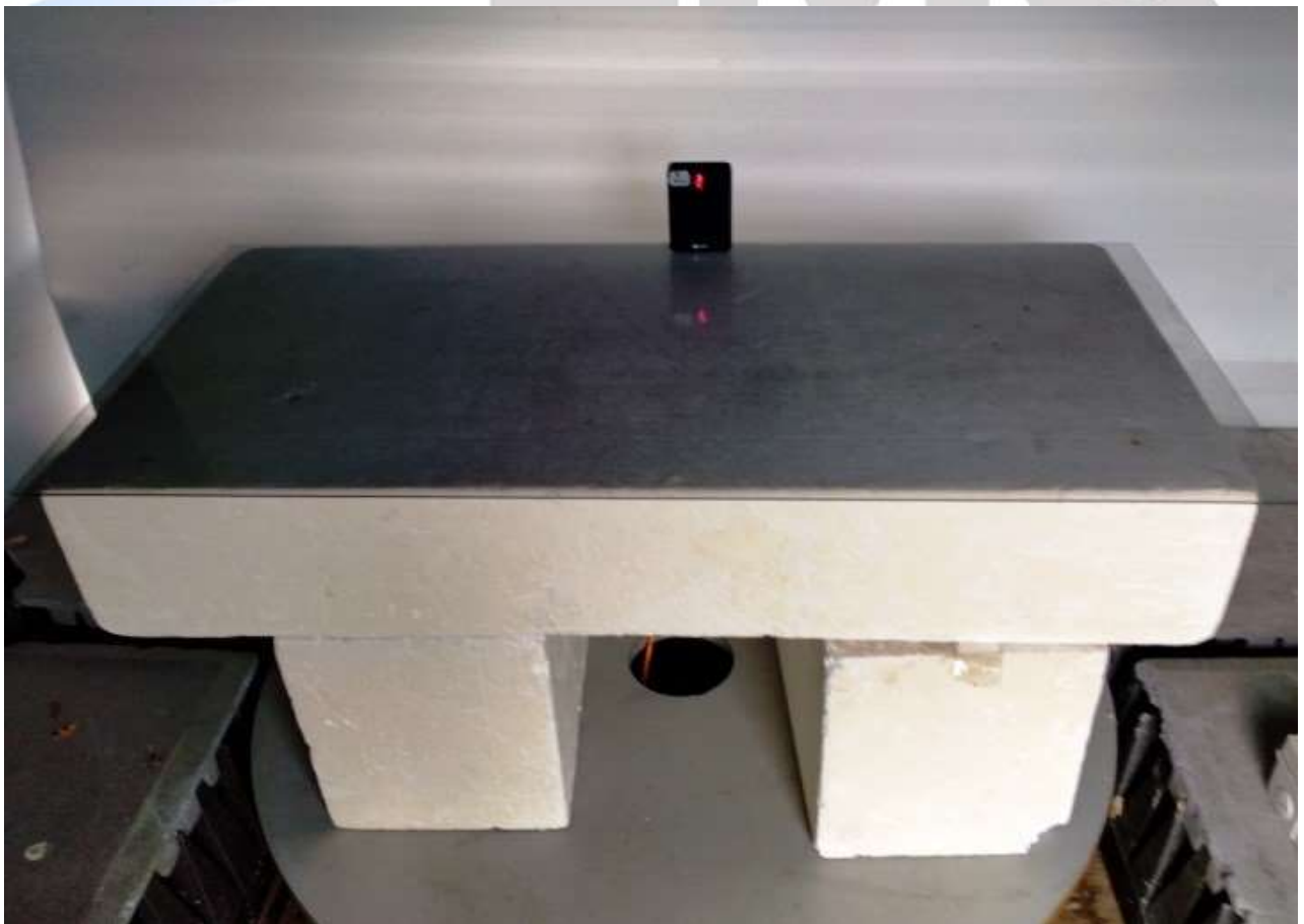
Radiated emissions test setup
