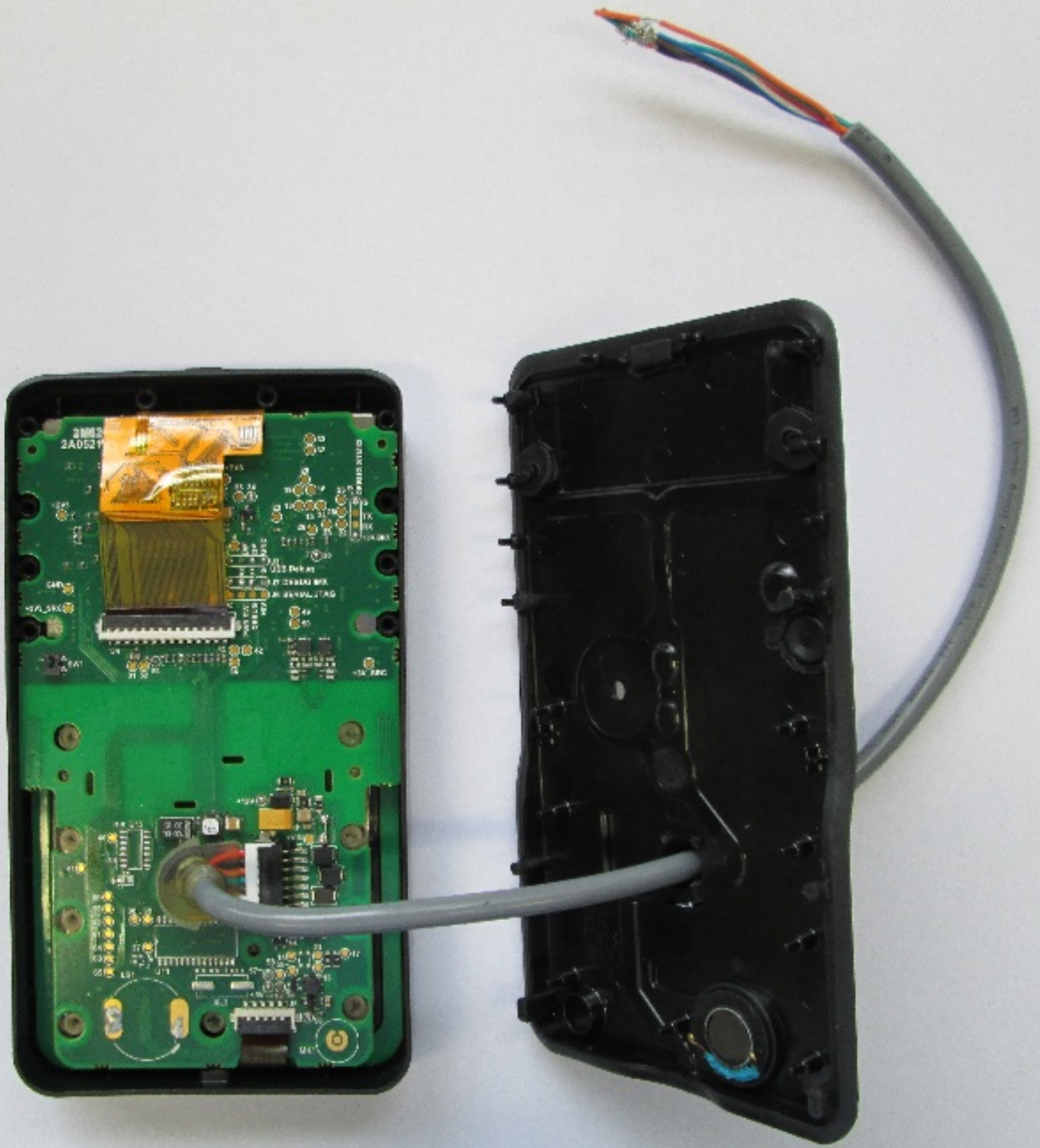
T20 Mifare - Internal Assembly 2
