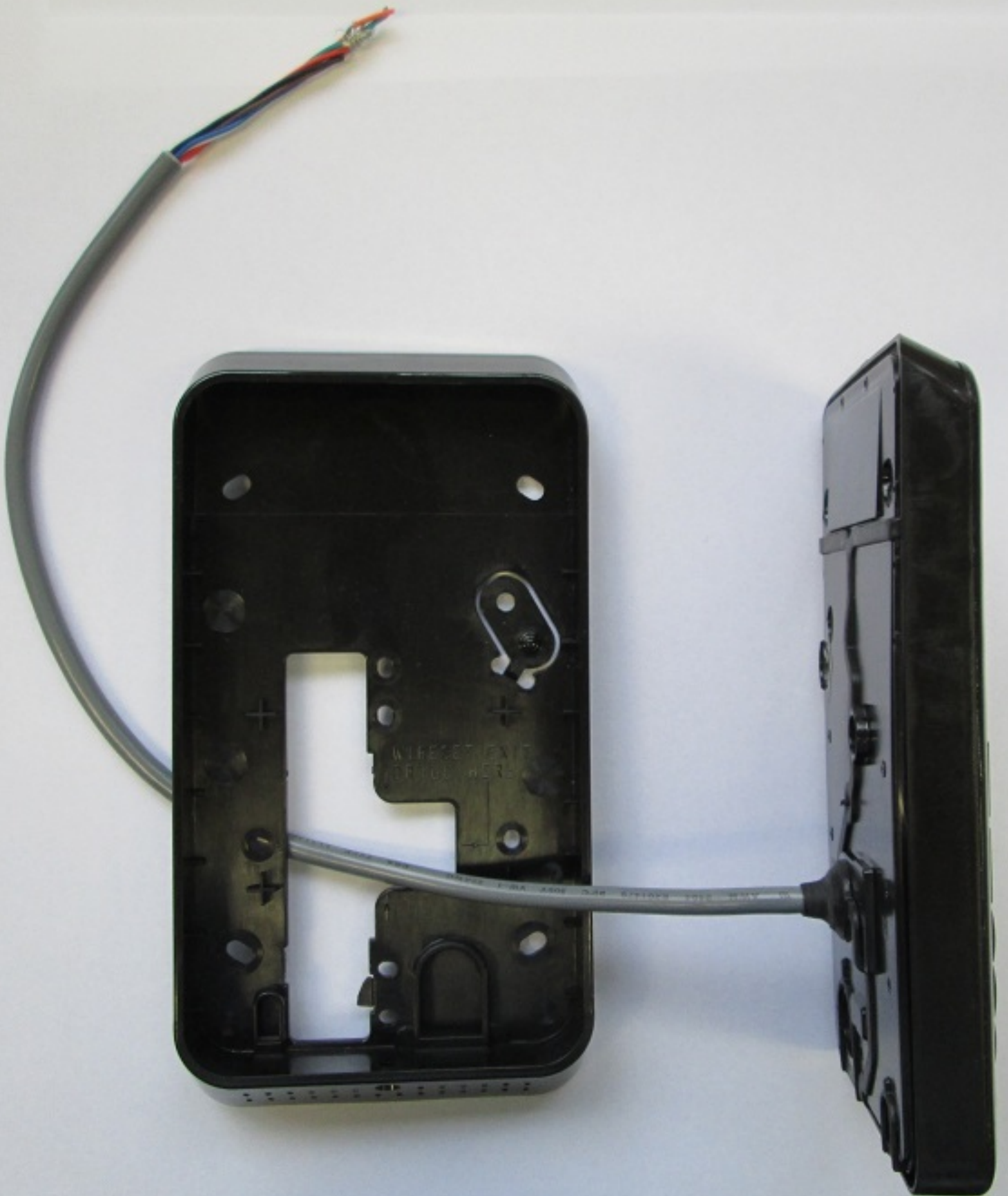
T20 Mifare Reader (Side View)
