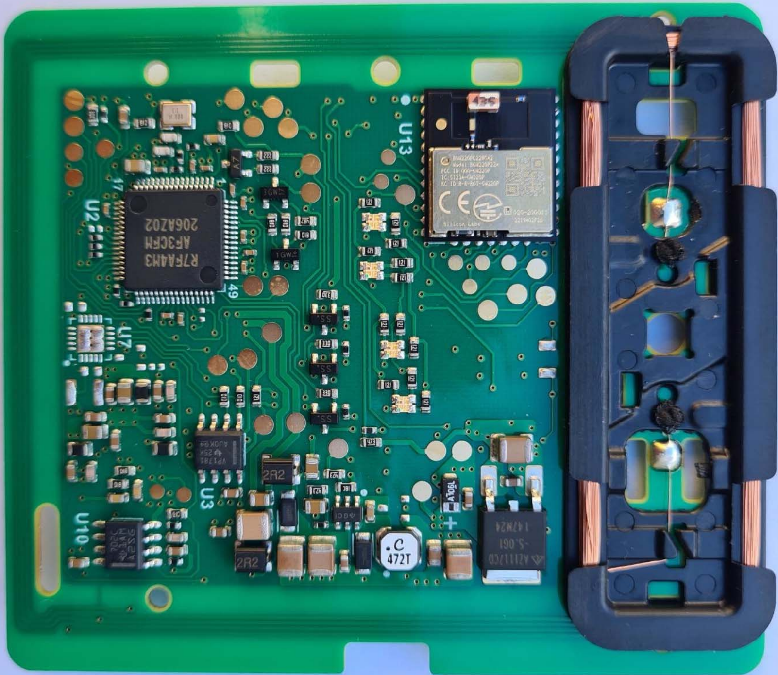
T12 Multi Tech - PCB (Front Side)
