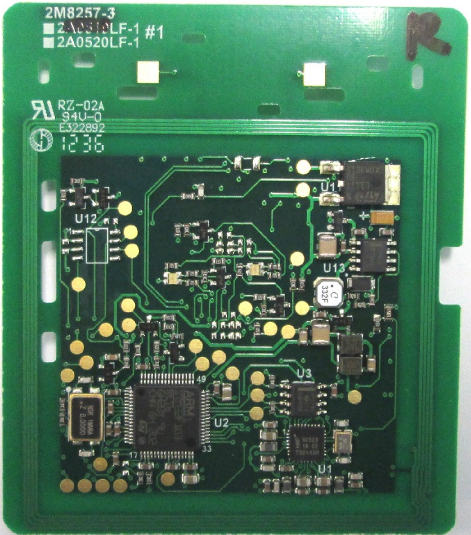
T12 Multi Tech - Antenna and PCB (Front Side)
