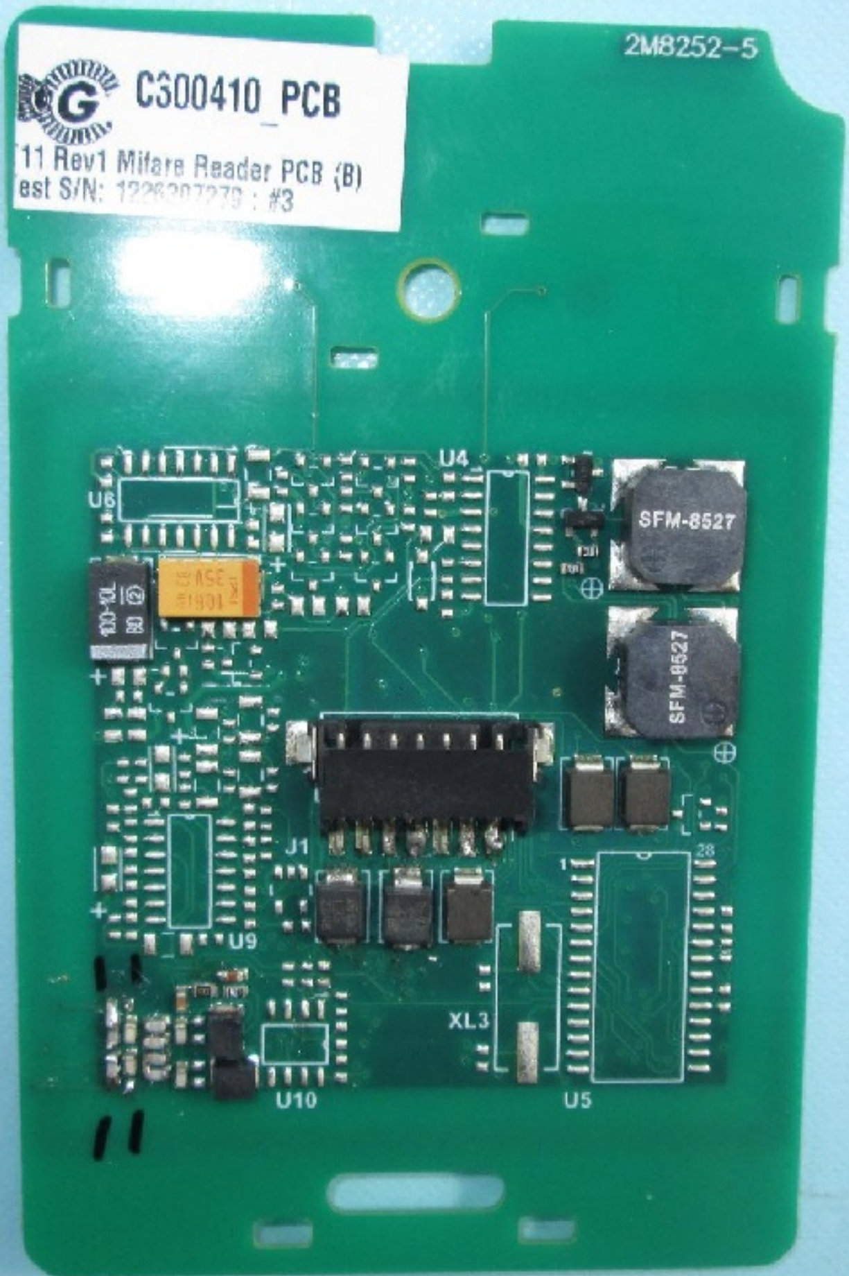
T11 Mifare - PCB (Rear Side)
