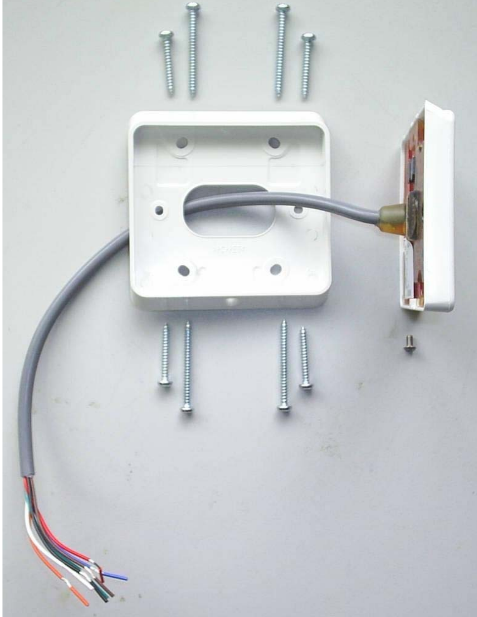
T12 Mifare - Assembly
