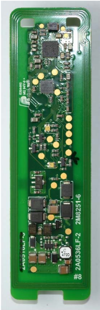
T10 Mifare - PCB (Front Side)
