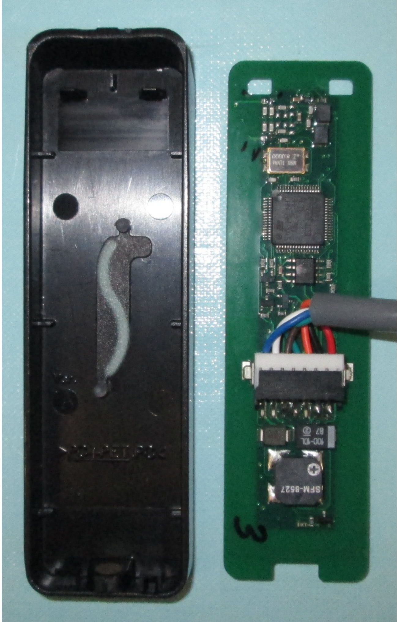
T10 Mifare - Front Cover and PCB Assembly
