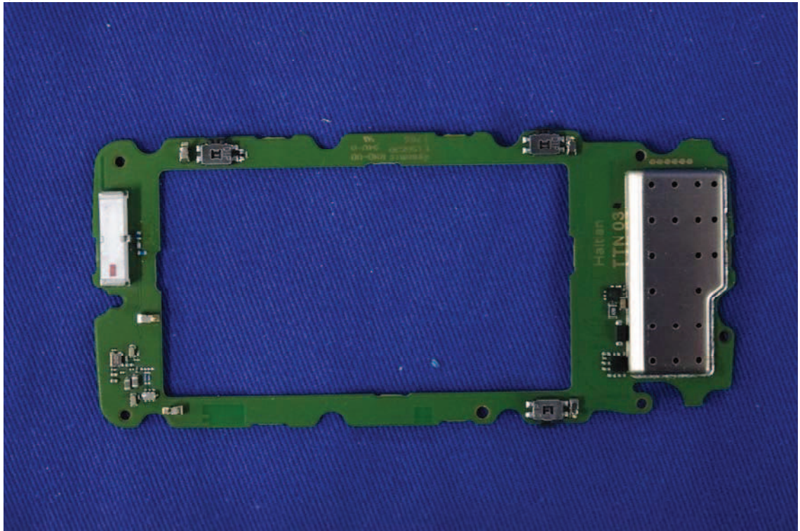
(23) EUT Photo
