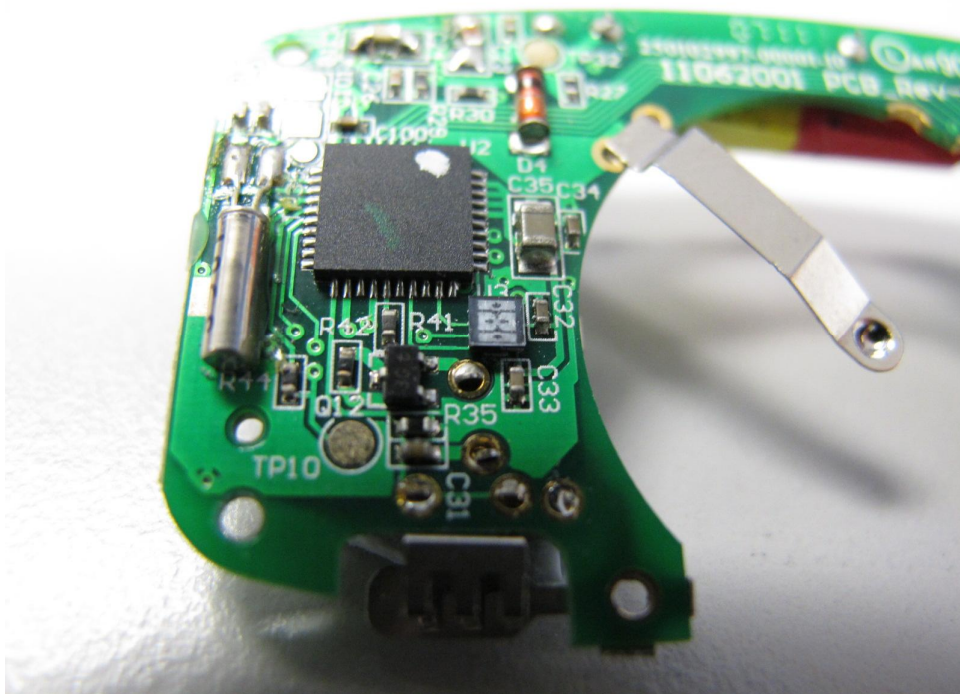
U3 – VTI CMA3000 (replaced part)
