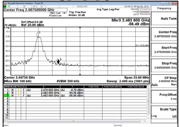
Band Edge_BLE_1M_HighCH39-2480
