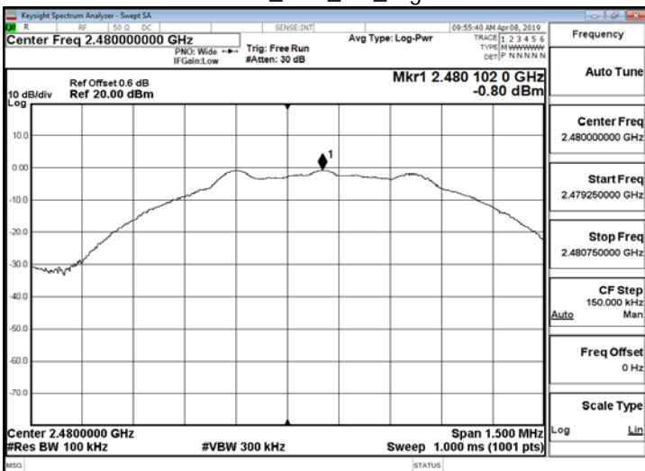
Reference Level_BLE_1M_HighCH39-2480
