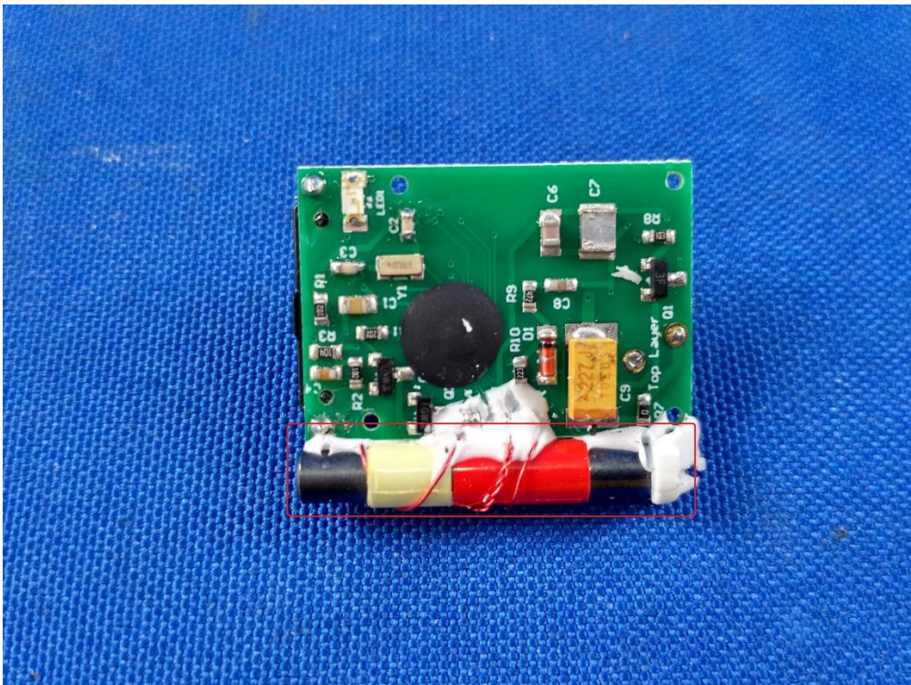
Antenna Position
