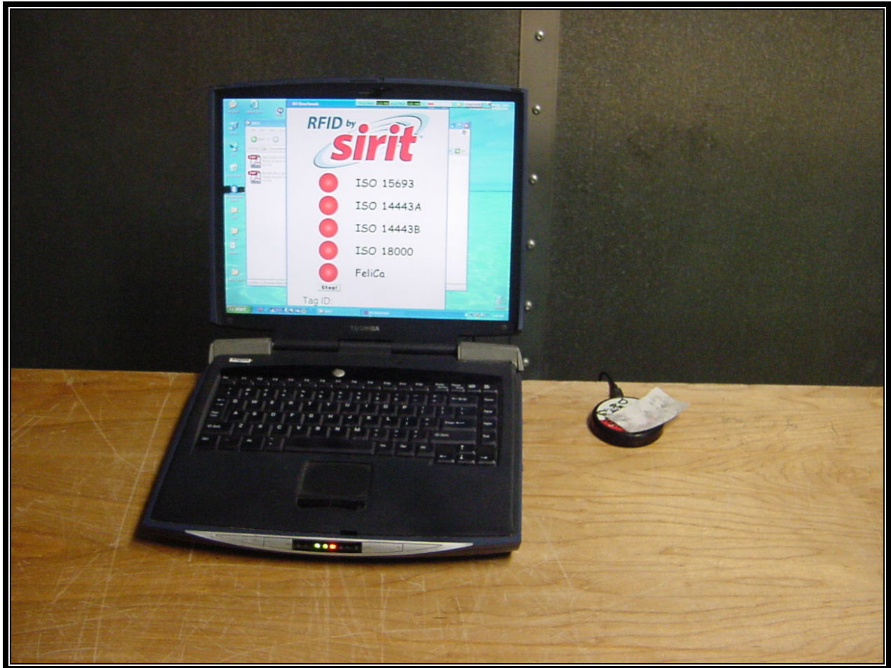
Photograph 4: Conducted AC Testing – Front View
