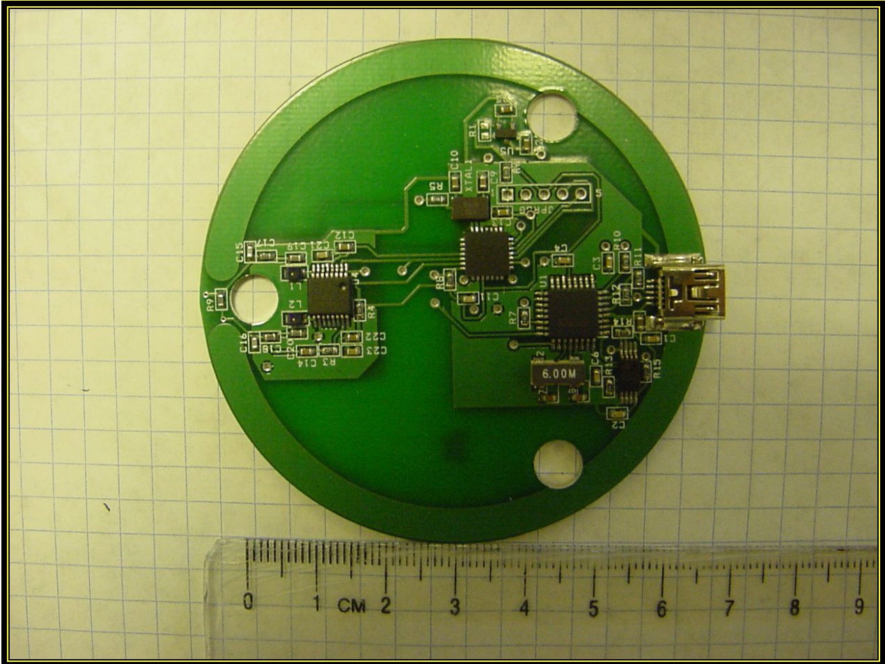
Photograph 9: Top of PCB
