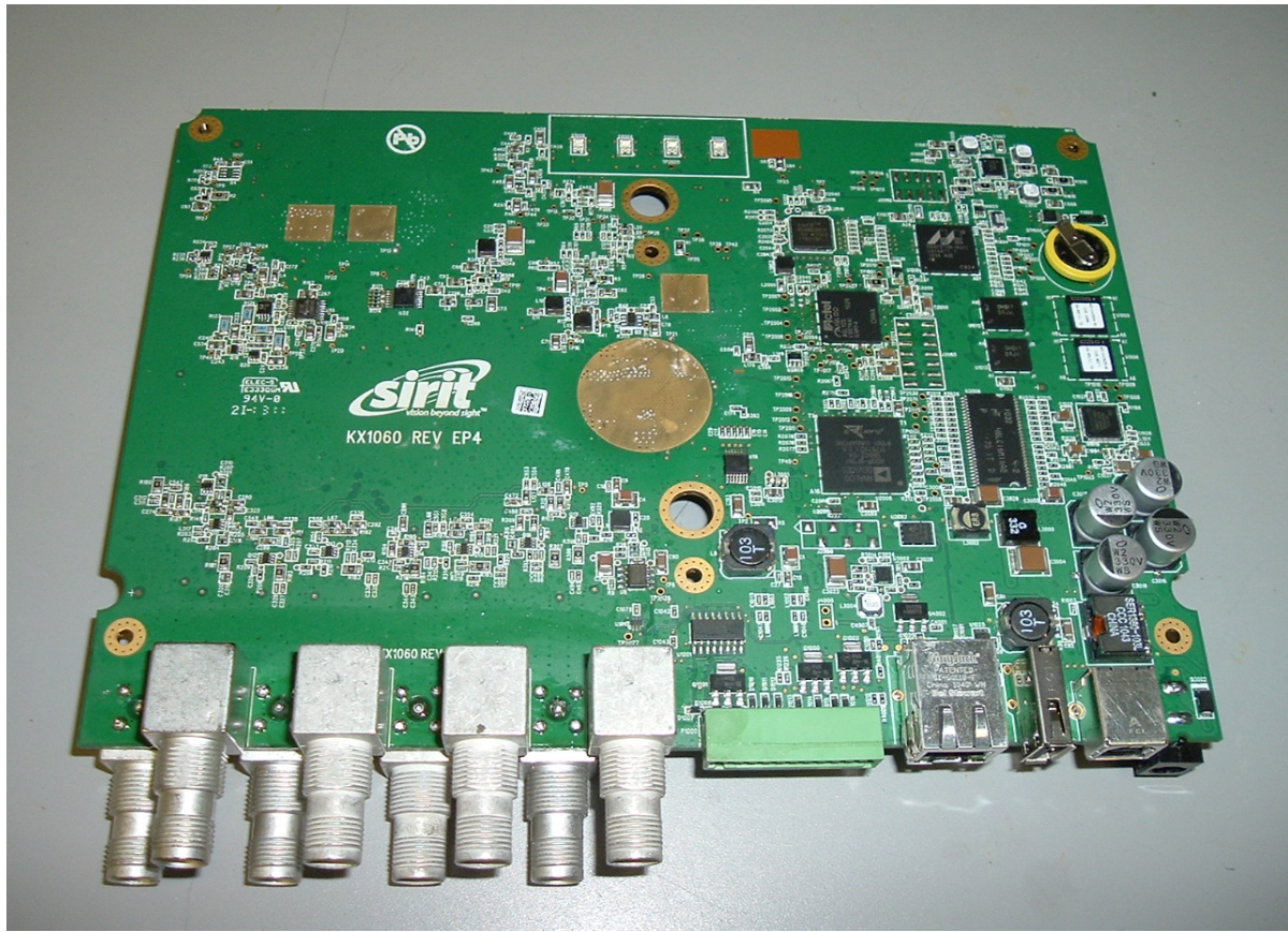
Printed Circuit Board, Top
