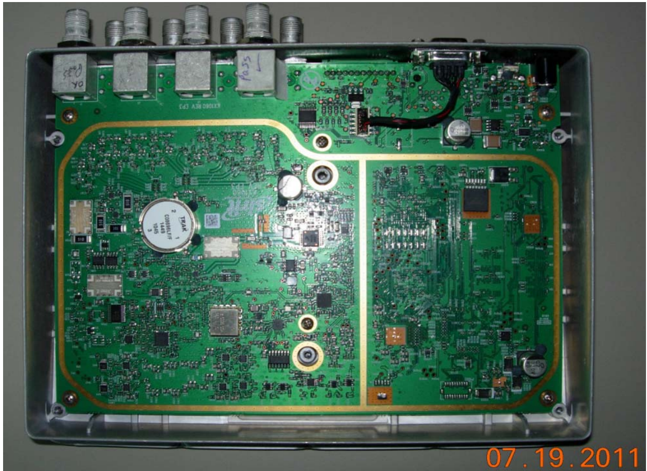
Printed Circuit Board Installed in Chassis Top
