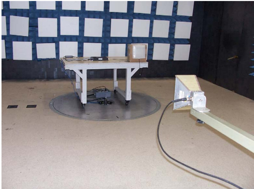
Figure 4 – View of radiated emissions from 1GHz to 10GHz
