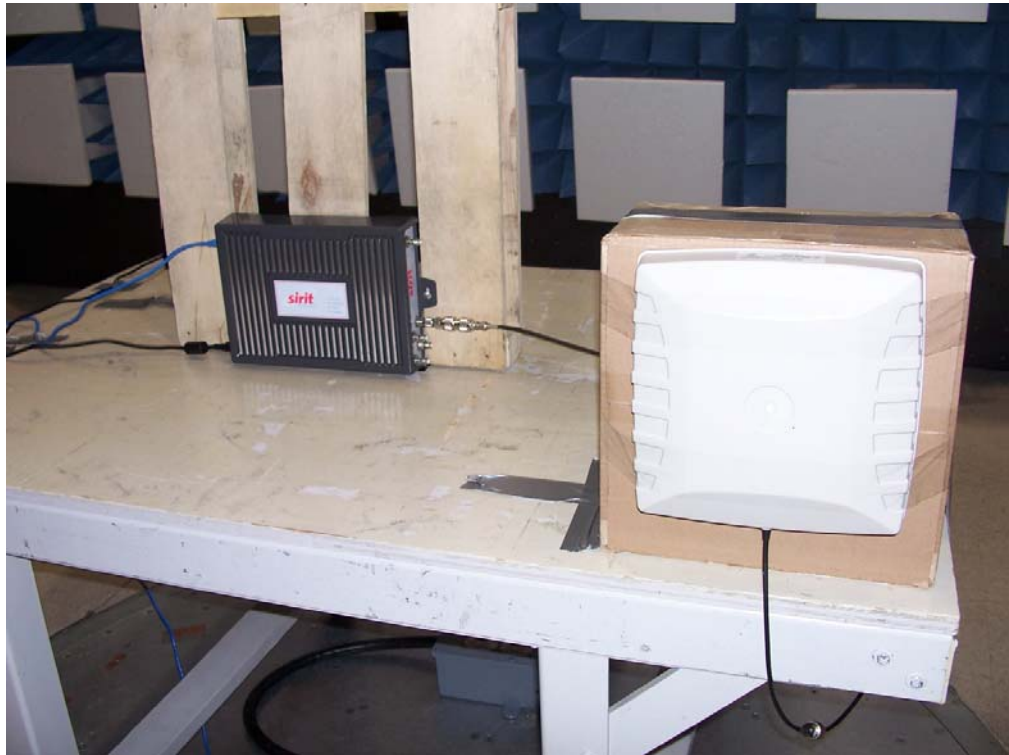
Figure 3 – Test setup investigating the EUT in different orientations.
