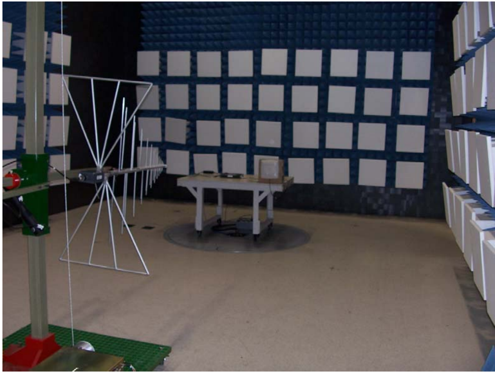
Figure 1 - Radiated Emissions Test Setup 30MHz – 1GHz
