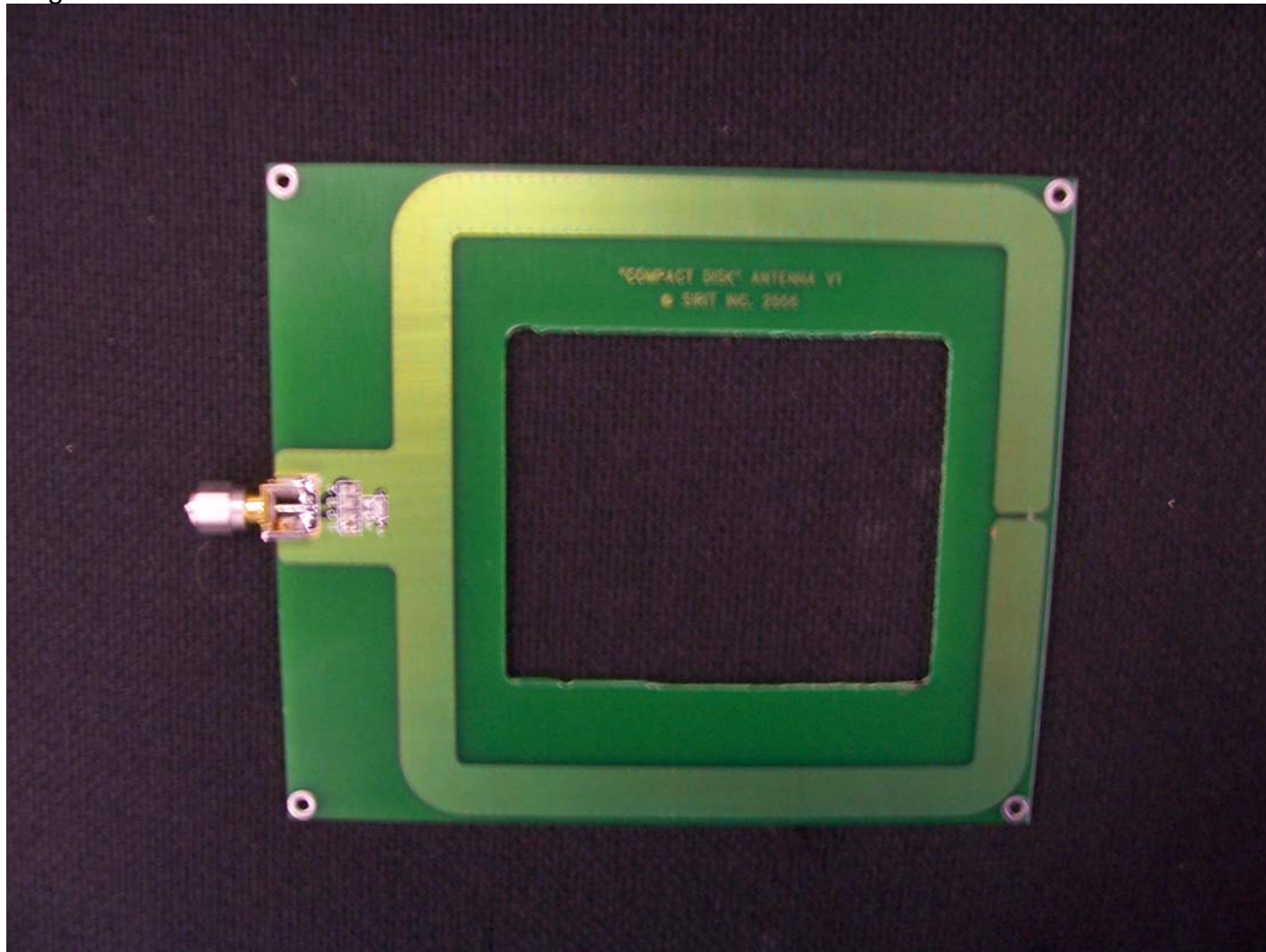
Large Antenna
