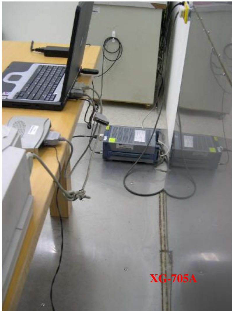
Photo 2: Conducted Emission Test Set-up
