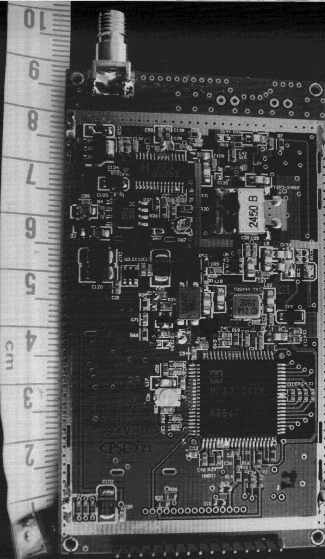
Disassembled View of RF Module (Back Side)
