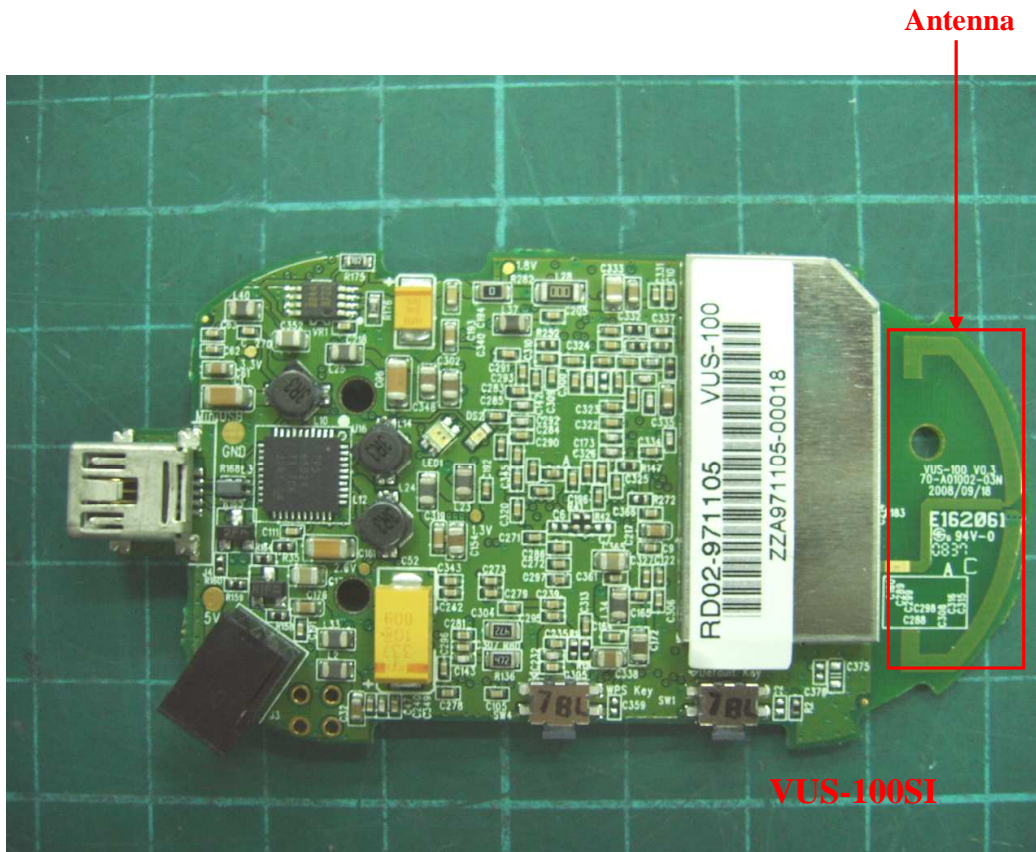
Photo 2: Internal photo of EUT
