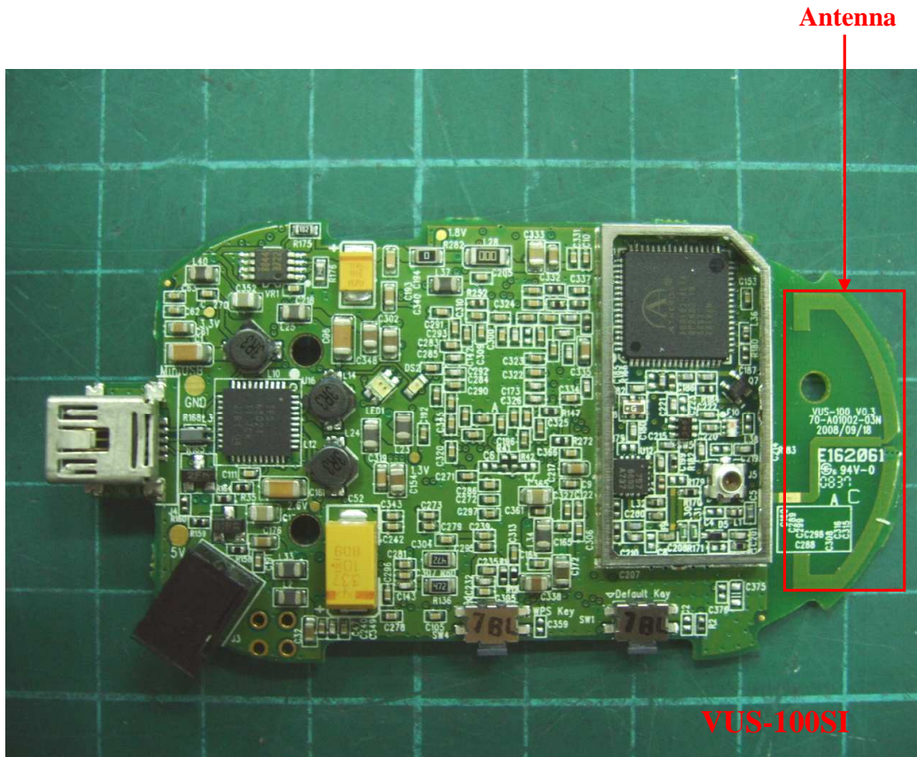
Photo 3: Internal photo of EUT
